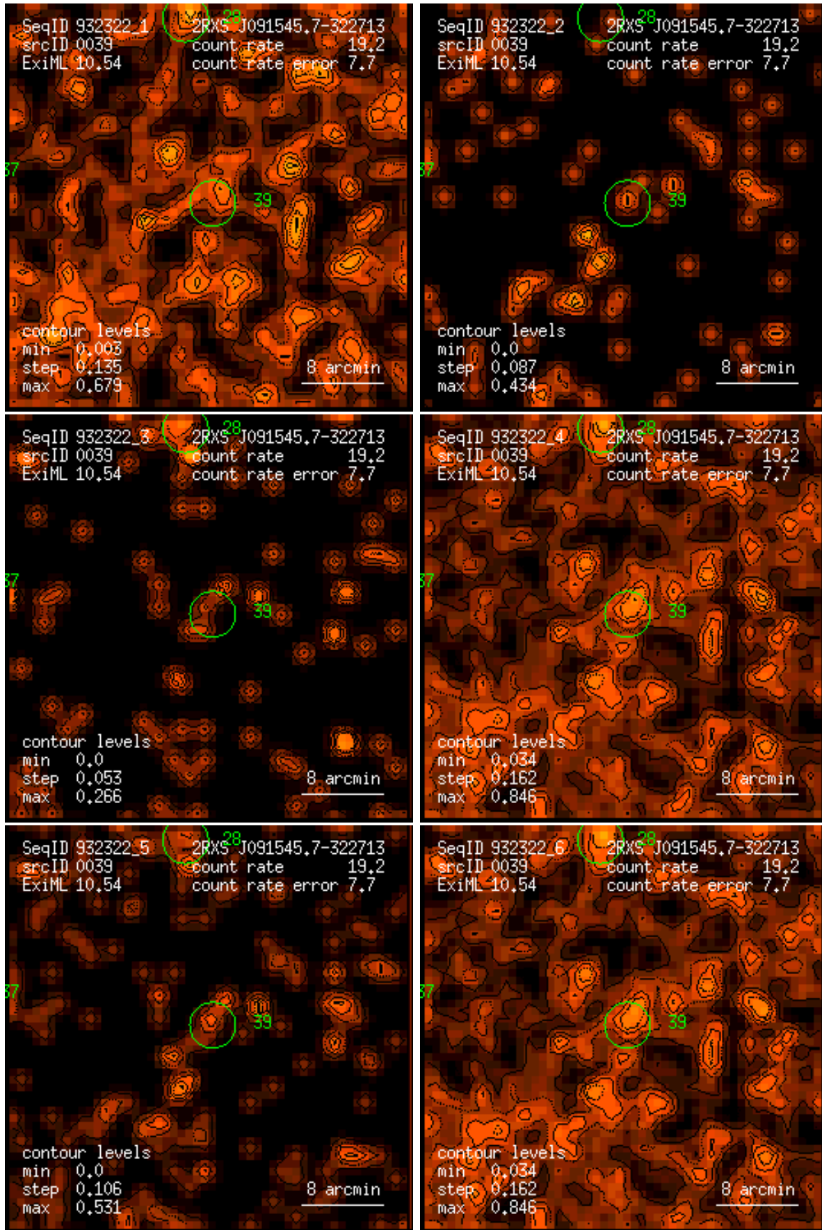
Figure 39: RASS 932322: detection 0039: band rate images, Gaussian filter: (1) PSPC channels 11 – 41, (2) 52 – 90, (3) 91 – 201, (4) 11 – 235, (5) 52 – 201, (6) 11 – 201. Broad band rates in counts/ks. Band rate contour levels in counts/ks/arcmin 2 .
