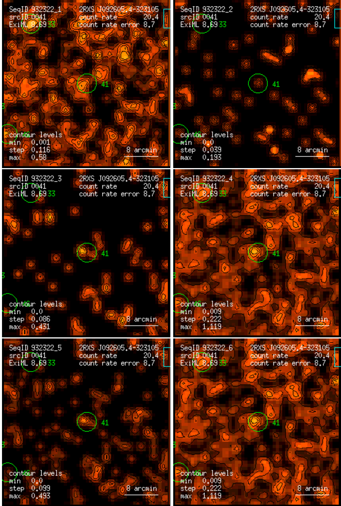
Figure 41: RASS 932322: detection 0041: band rate images, Gaussian filter: (1) PSPC channels 11 – 41, (2) 52 – 90, (3) 91 – 201, (4) 11 – 235, (5) 52 – 201, (6) 11 – 201. Broad band rates in counts/ks. Band rate contour levels in counts/ks/arcmin 2 .
