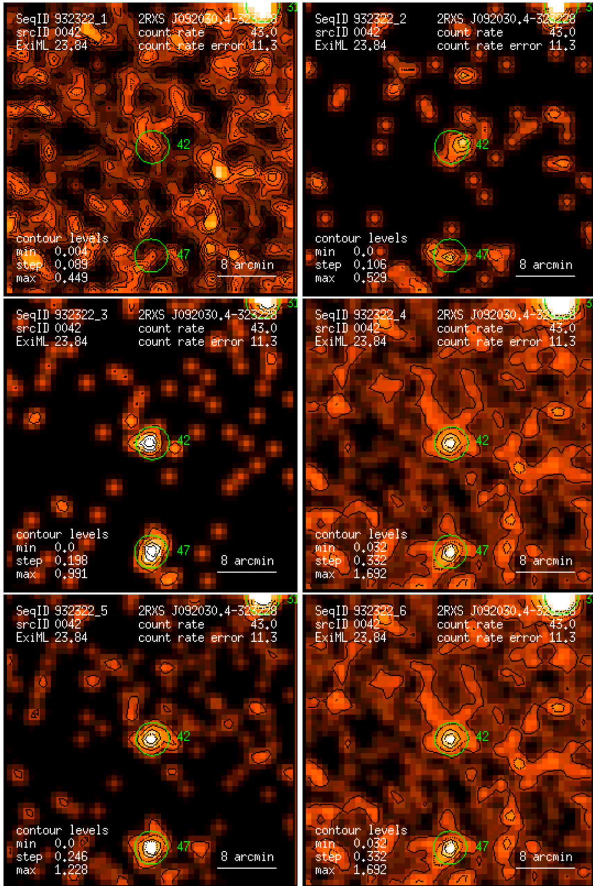
Figure 42: RASS 932322: detection 0042: band rate images, Gaussian filter: (1) PSPC channels 11 – 41, (2) 52 – 90, (3) 91 – 201, (4) 11 – 235, (5) 52 – 201, (6) 11 – 201. Broad band rates in counts/ks. Band rate contour levels in counts/ks/arcmin 2 .
