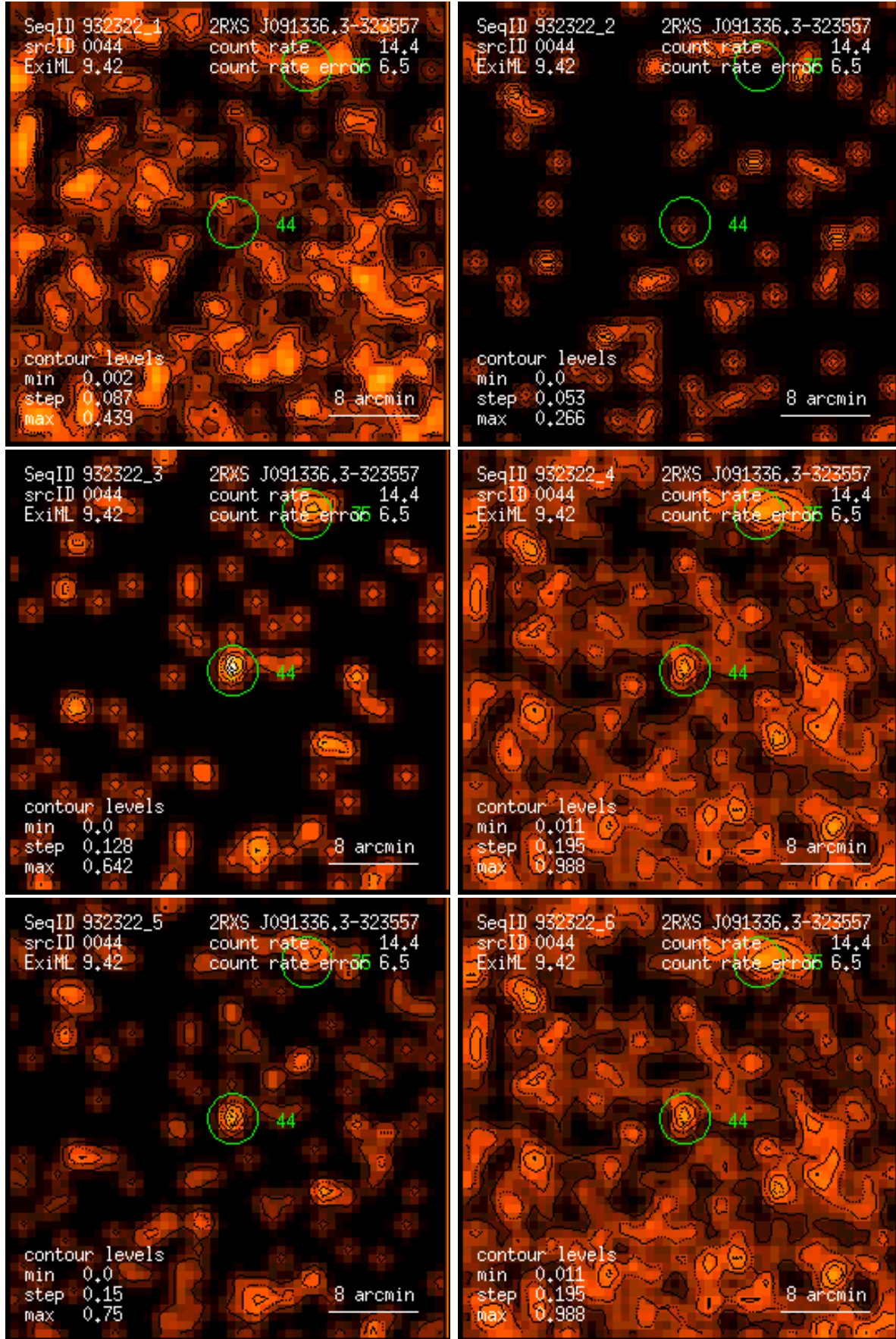
Figure 44: RASS 932322: detection 0044: band rate images, Gaussian filter: (1) PSPC channels 11 – 41, (2) 52 – 90, (3) 91 – 201, (4) 11 – 235, (5) 52 – 201, (6) 11 – 201. Broad band rates in counts/ks. Band rate contour levels in counts/ks/arcmin 2 .
