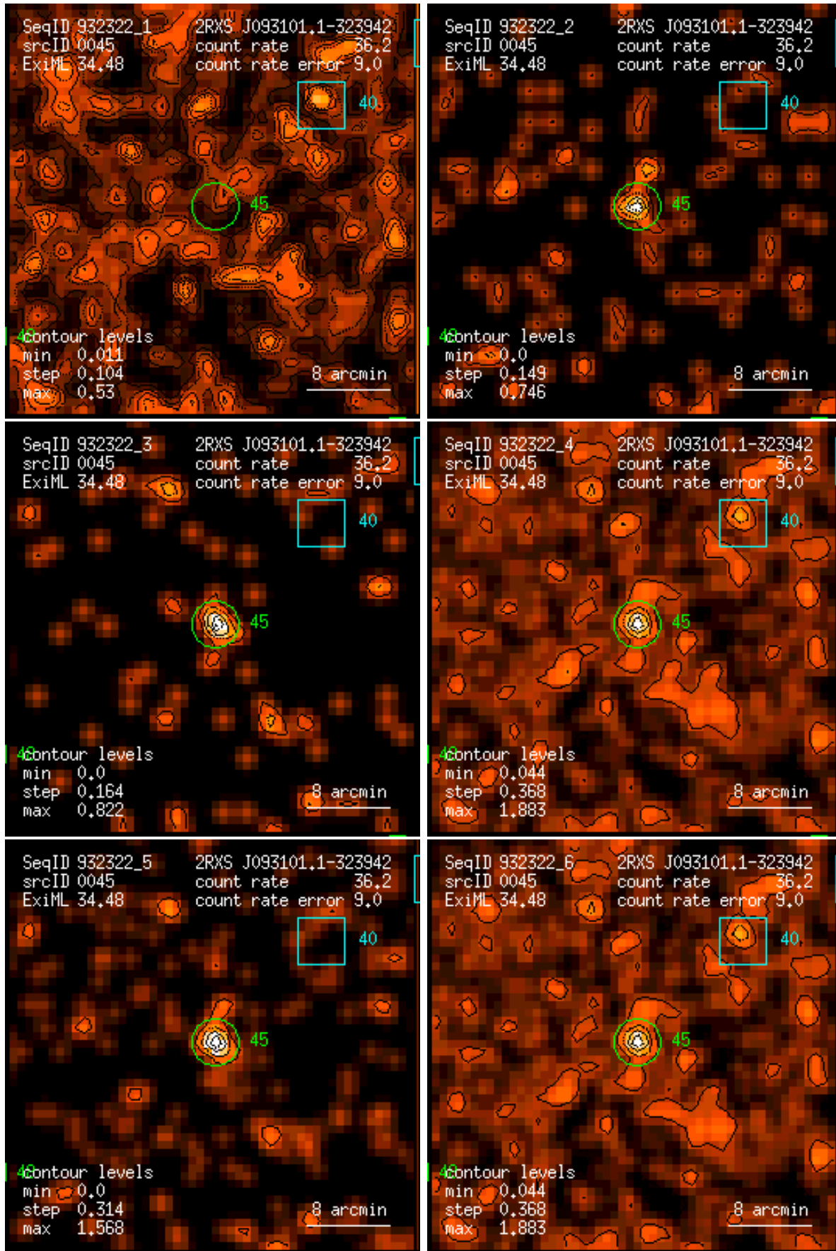
Figure 45: RASS 932322: detection 0045: band rate images, Gaussian filter: (1) PSPC channels 11 – 41, (2) 52 – 90, (3) 91 – 201, (4) 11 – 235, (5) 52 – 201, (6) 11 – 201. Broad band rates in counts/ks. Band rate contour levels in counts/ks/arcmin 2 .
