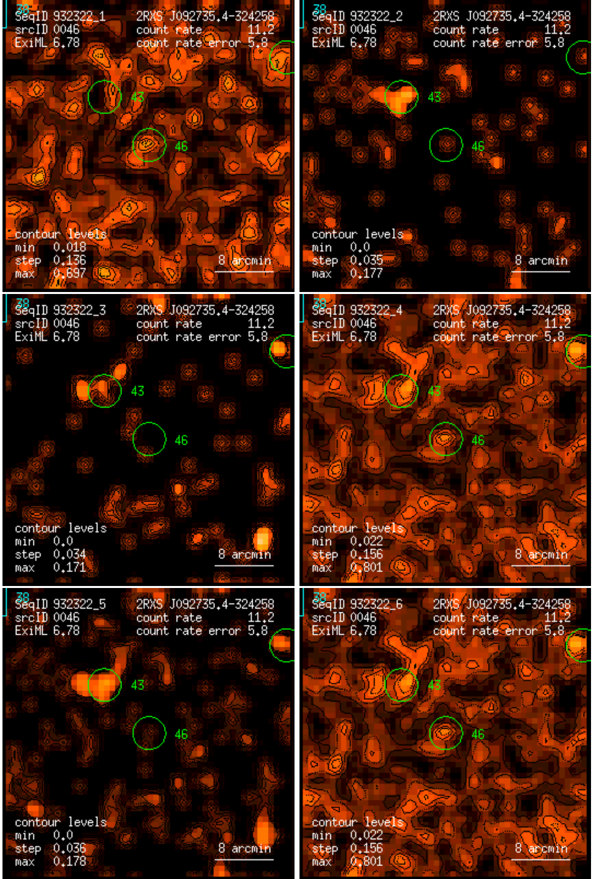
Figure 46: RASS 932322: detection 0046: band rate images, Gaussian filter: (1) PSPC channels 11 – 41, (2) 52 – 90, (3) 91 – 201, (4) 11 – 235, (5) 52 – 201, (6) 11 – 201. Broad band rates in counts/ks. Band rate contour levels in counts/ks/arcmin 2 .
