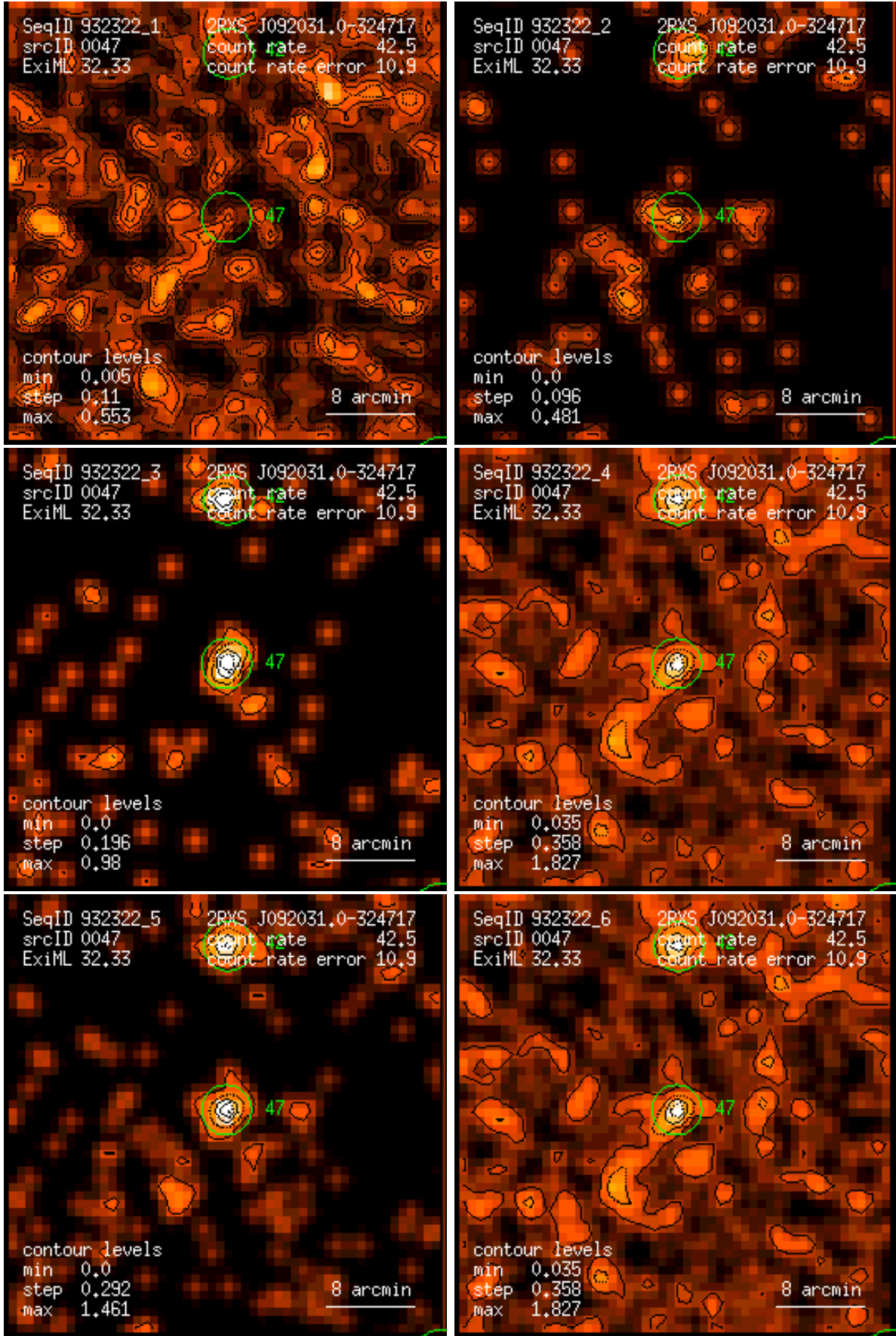
Figure 47: RASS 932322: detection 0047: band rate images, Gaussian filter: (1) PSPC channels 11 – 41, (2) 52 – 90, (3) 91 – 201, (4) 11 – 235, (5) 52 – 201, (6) 11 – 201. Broad band rates in counts/ks. Band rate contour levels in counts/ks/arcmin 2 .
