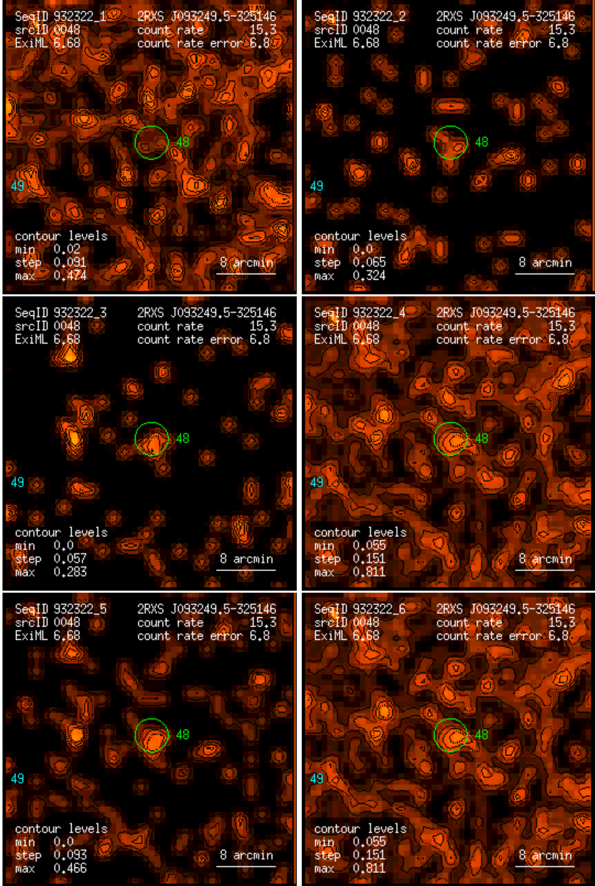
Figure 48: RASS 932322: detection 0048: band rate images, Gaussian filter: (1) PSPC channels 11 – 41, (2) 52 – 90, (3) 91 – 201, (4) 11 – 235, (5) 52 – 201, (6) 11 – 201. Broad band rates in counts/ks. Band rate contour levels in counts/ks/arcmin 2 .
