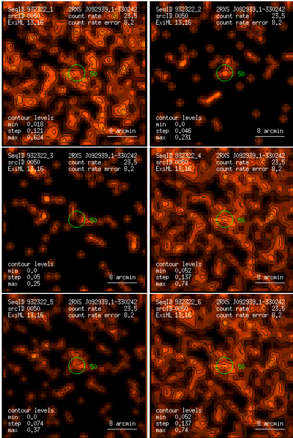
Figure 50: RASS 932322: detection 0050: band rate images, Gaussian filter: (1) PSPC channels 11 – 41, (2) 52 – 90, (3) 91 – 201, (4) 11 – 235, (5) 52 – 201, (6) 11 – 201. Broad band rates in counts/ks. Band rate contour levels in counts/ks/arcmin 2 .
