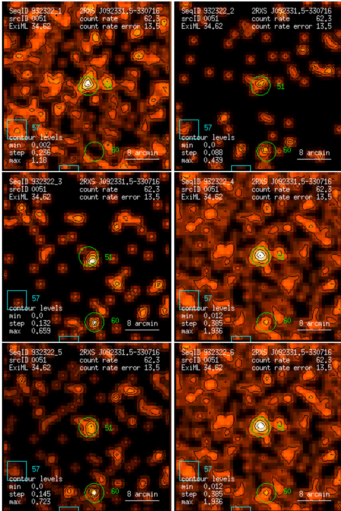
Figure 51: RASS 932322: detection 0051: band rate images, Gaussian filter: (1) PSPC channels 11 – 41, (2) 52 – 90, (3) 91 – 201, (4) 11 – 235, (5) 52 – 201, (6) 11 – 201. Broad band rates in counts/ks. Band rate contour levels in counts/ks/arcmin 2 .
