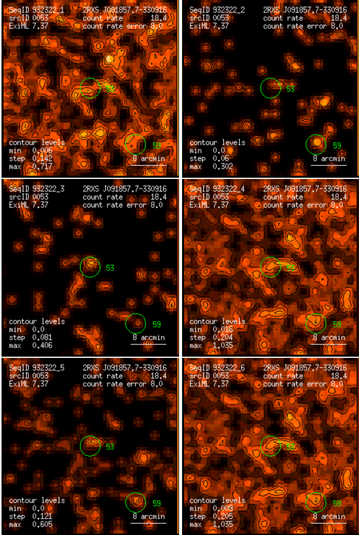
Figure 53: RASS 932322: detection 0053: band rate images, Gaussian filter: (1) PSPC channels 11 – 41, (2) 52 – 90, (3) 91 – 201, (4) 11 – 235, (5) 52 – 201, (6) 11 – 201. Broad band rates in counts/ks. Band rate contour levels in counts/ks/arcmin 2 .
