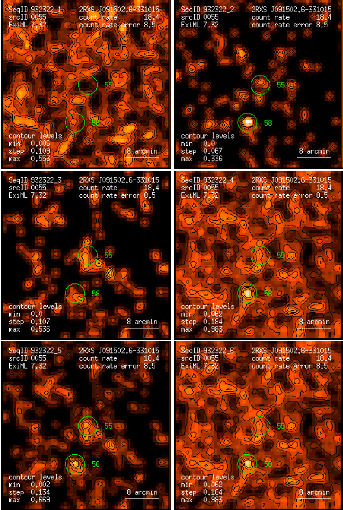
Figure 55: RASS 932322: detection 0055: band rate images, Gaussian filter: (1) PSPC channels 11 – 41, (2) 52 – 90, (3) 91 – 201, (4) 11 – 235, (5) 52 – 201, (6) 11 – 201. Broad band rates in counts/ks. Band rate contour levels in counts/ks/arcmin 2 .
