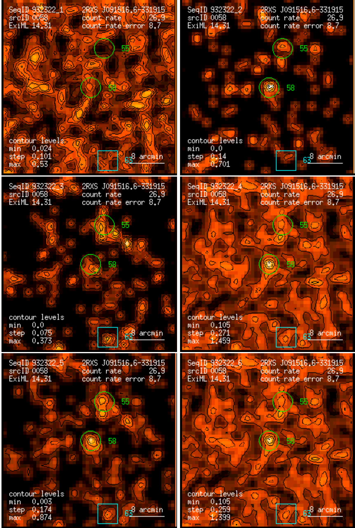
Figure 58: RASS 932322: detection 0058: band rate images, Gaussian filter: (1) PSPC channels 11 – 41, (2) 52 – 90, (3) 91 – 201, (4) 11 – 235, (5) 52 – 201, (6) 11 – 201. Broad band rates in counts/ks. Band rate contour levels in counts/ks/arcmin 2 .
