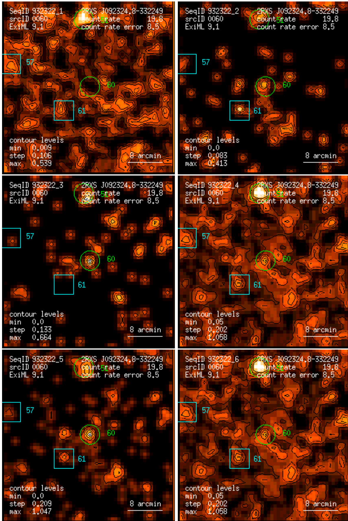
Figure 60: RASS 932322: detection 0060: band rate images, Gaussian filter: (1) PSPC channels 11 – 41, (2) 52 – 90, (3) 91 – 201, (4) 11 – 235, (5) 52 – 201, (6) 11 – 201. Broad band rates in counts/ks. Band rate contour levels in counts/ks/arcmin 2 .
