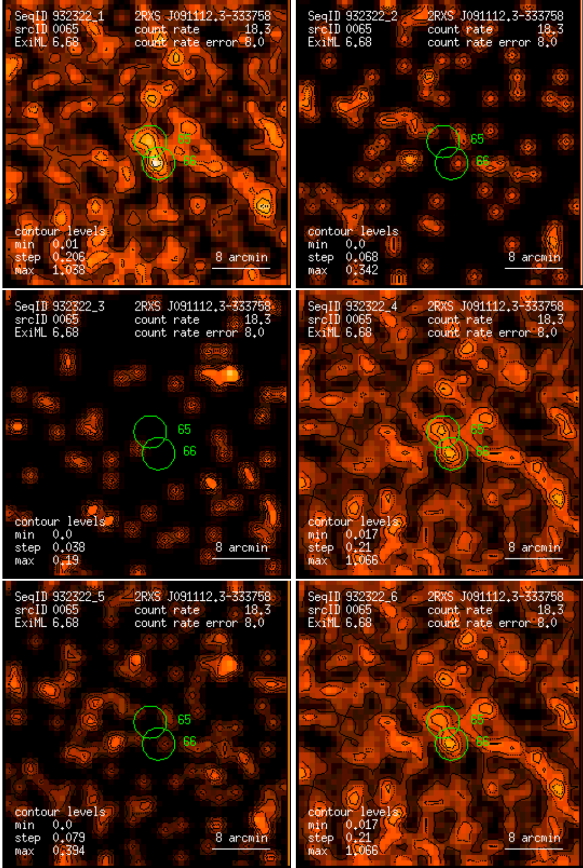
Figure 65: RASS 932322: detection 0065: band rate images, Gaussian filter: (1) PSPC channels 11 – 41, (2) 52 – 90, (3) 91 – 201, (4) 11 – 235, (5) 52 – 201, (6) 11 – 201. Broad band rates in counts/ks. Band rate contour levels in counts/ks/arcmin 2 .
