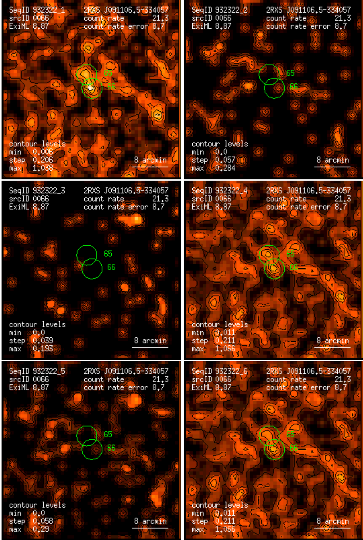
Figure 66: RASS 932322: detection 0066: band rate images, Gaussian filter: (1) PSPC channels 11 – 41, (2) 52 – 90, (3) 91 – 201, (4) 11 – 235, (5) 52 – 201, (6) 11 – 201. Broad band rates in counts/ks. Band rate contour levels in counts/ks/arcmin 2 .
