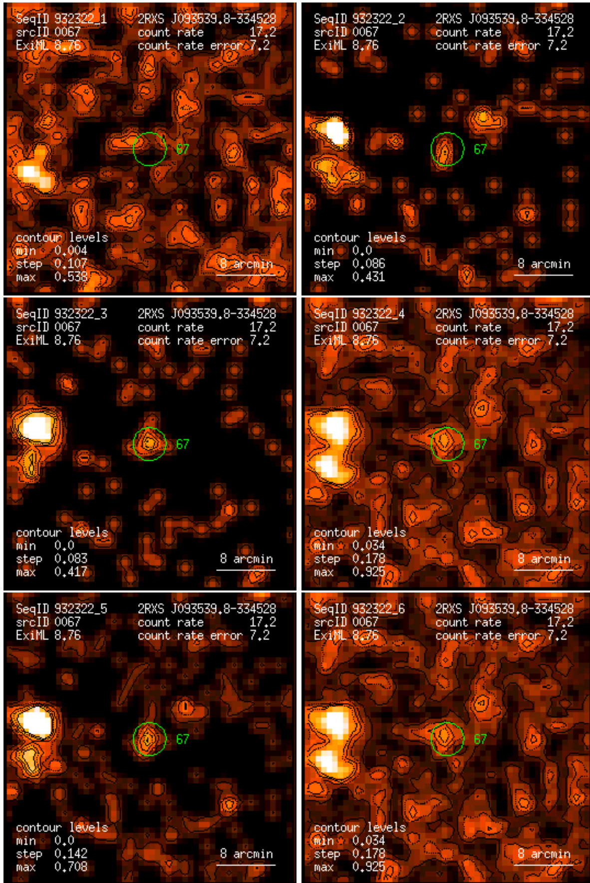
Figure 67: RASS 932322: detection 0067: band rate images, Gaussian filter: (1) PSPC channels 11 – 41, (2) 52 – 90, (3) 91 – 201, (4) 11 – 235, (5) 52 – 201, (6) 11 – 201. Broad band rates in counts/ks. Band rate contour levels in counts/ks/arcmin 2 .
