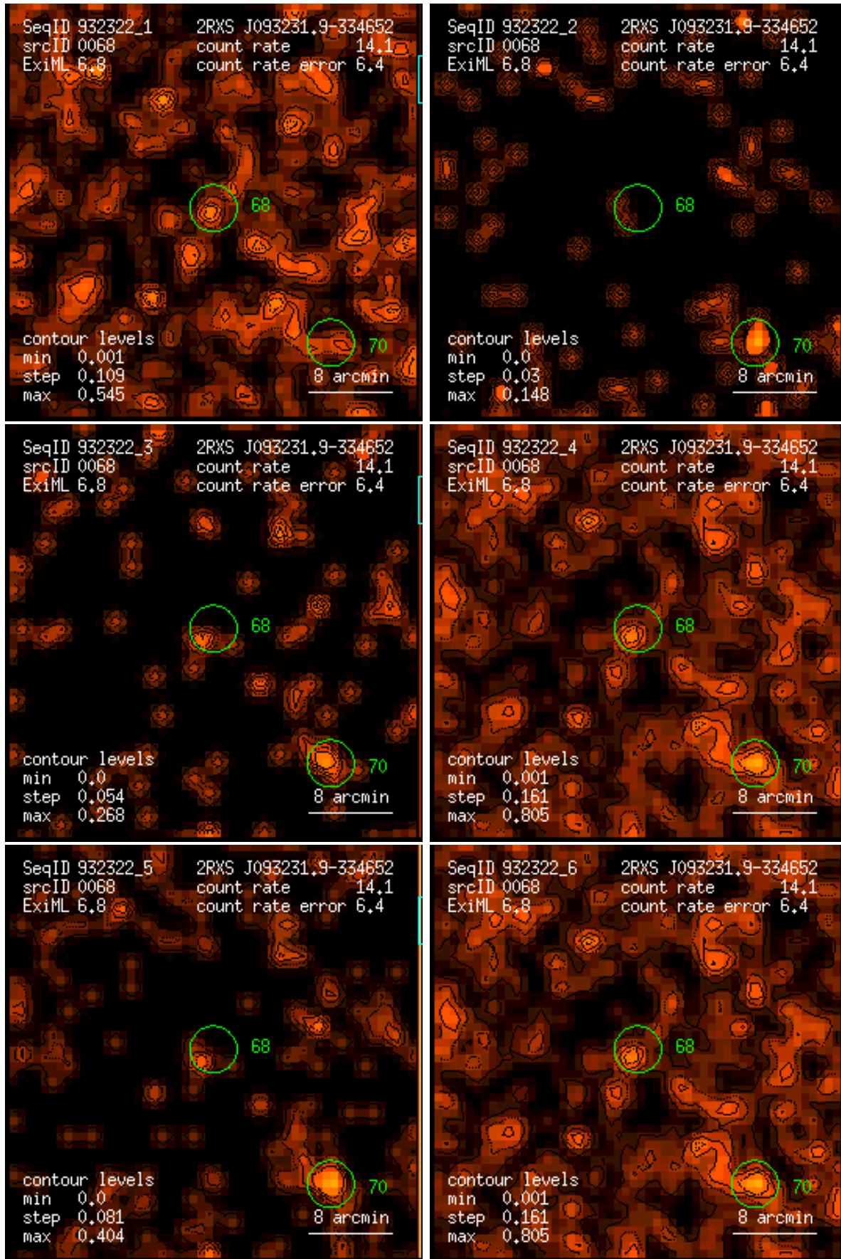
Figure 68: RASS 932322: detection 0068: band rate images, Gaussian filter: (1) PSPC channels 11 – 41, (2) 52 – 90, (3) 91 – 201, (4) 11 – 235, (5) 52 – 201, (6) 11 – 201. Broad band rates in counts/ks. Band rate contour levels in counts/ks/arcmin 2 .
