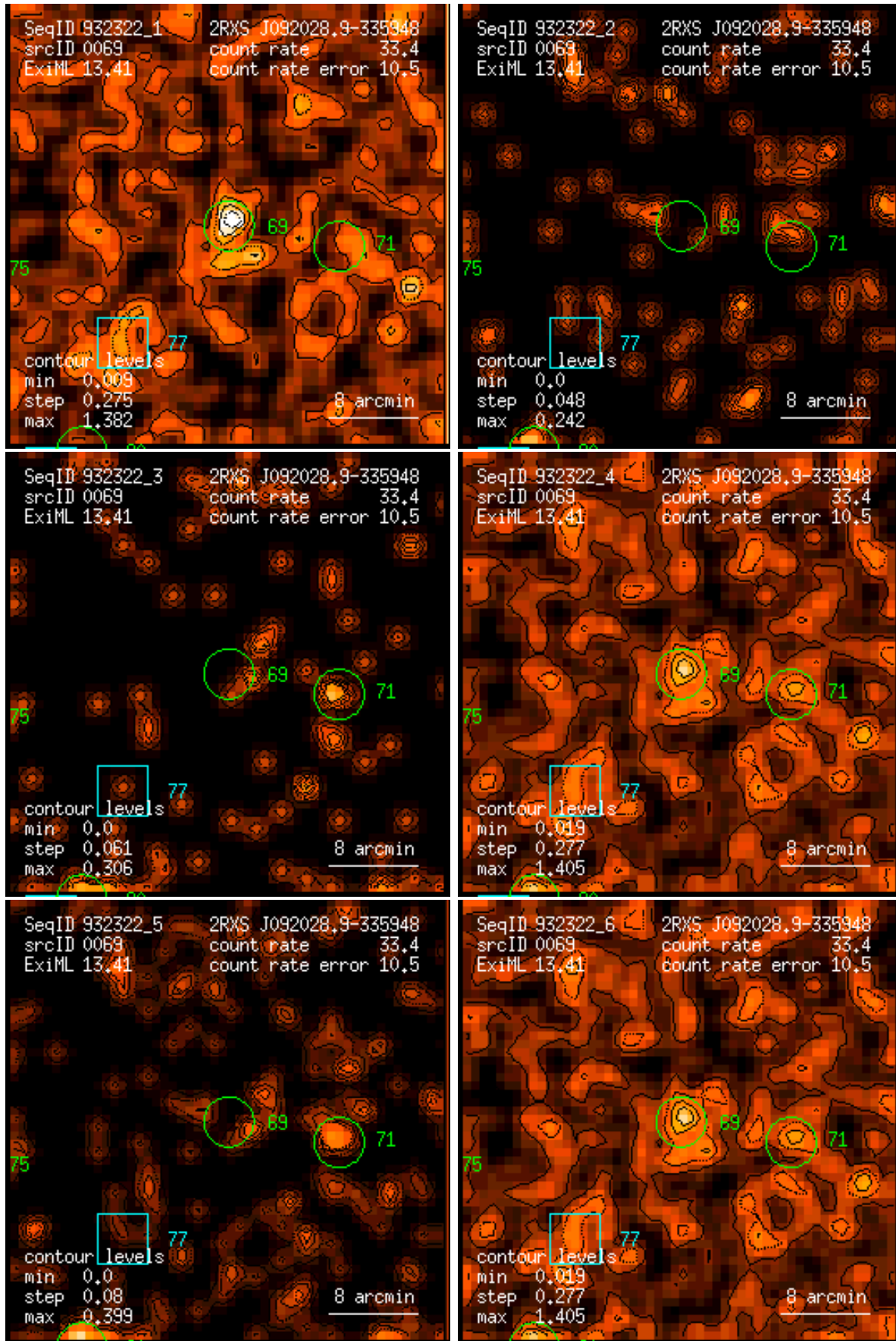
Figure 69: RASS 932322: detection 0069: band rate images, Gaussian filter: (1) PSPC channels 11 – 41, (2) 52 – 90, (3) 91 – 201, (4) 11 – 235, (5) 52 – 201, (6) 11 – 201. Broad band rates in counts/ks. Band rate contour levels in counts/ks/arcmin 2 .
