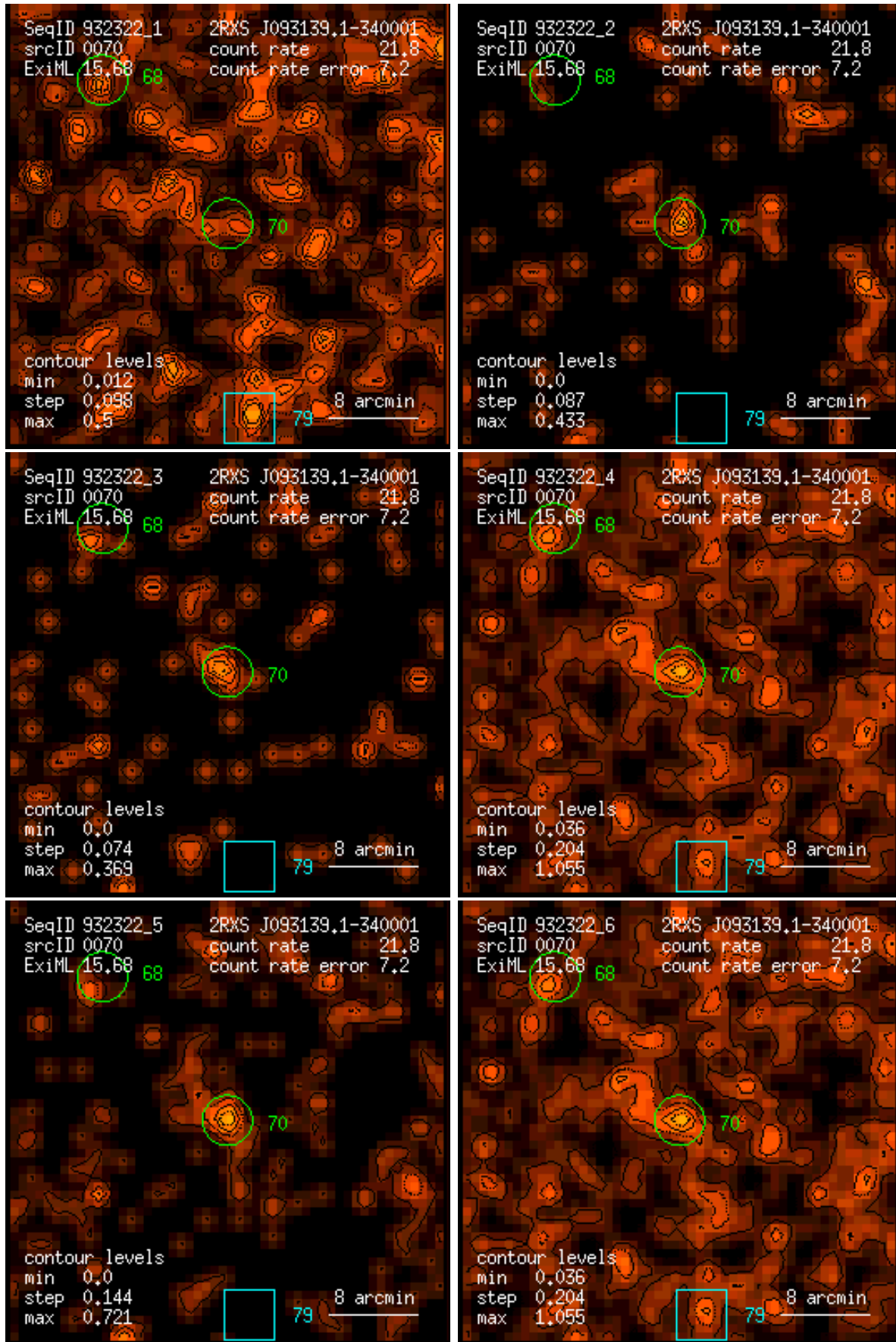
Figure 70: RASS 932322: detection 0070: band rate images, Gaussian filter: (1) PSPC channels 11 – 41, (2) 52 – 90, (3) 91 – 201, (4) 11 – 235, (5) 52 – 201, (6) 11 – 201. Broad band rates in counts/ks. Band rate contour levels in counts/ks/arcmin 2 .
