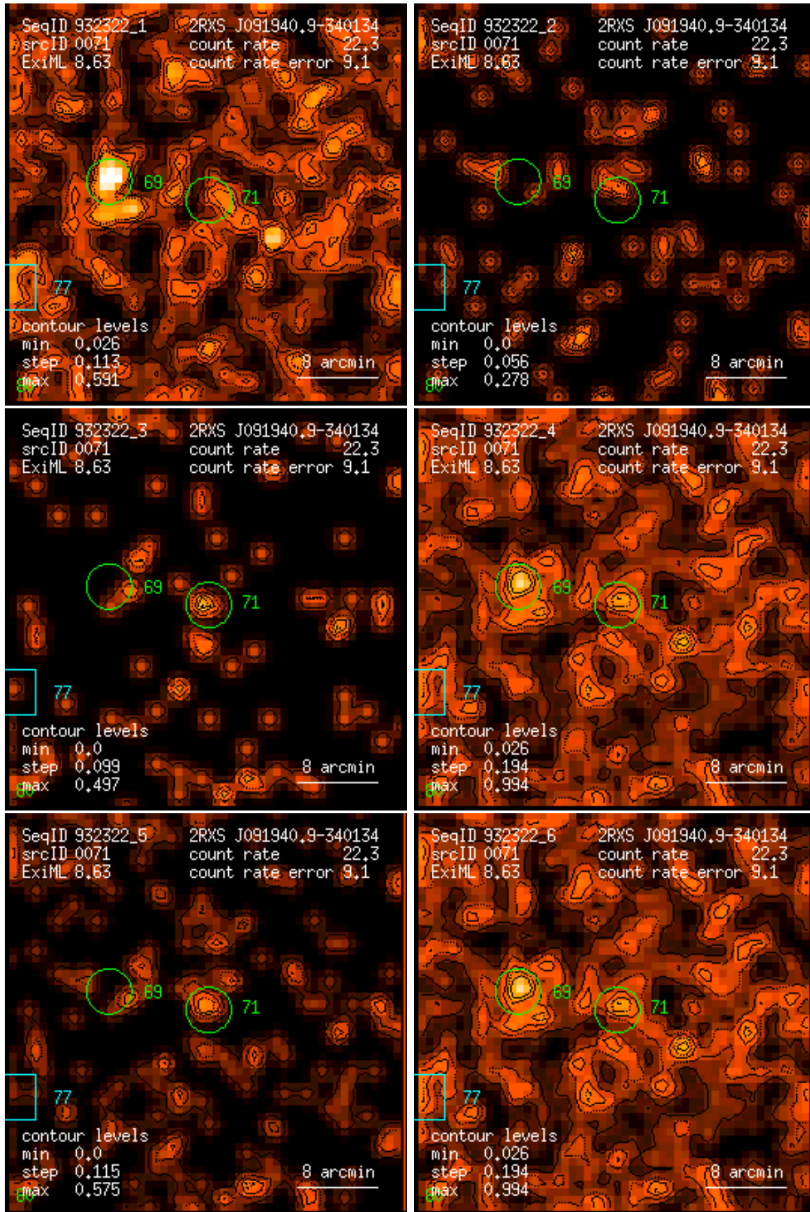
Figure 71: RASS 932322: detection 0071: band rate images, Gaussian filter: (1) PSPC channels 11 – 41, (2) 52 – 90, (3) 91 – 201, (4) 11 – 235, (5) 52 – 201, (6) 11 – 201. Broad band rates in counts/ks. Band rate contour levels in counts/ks/arcmin 2 .
