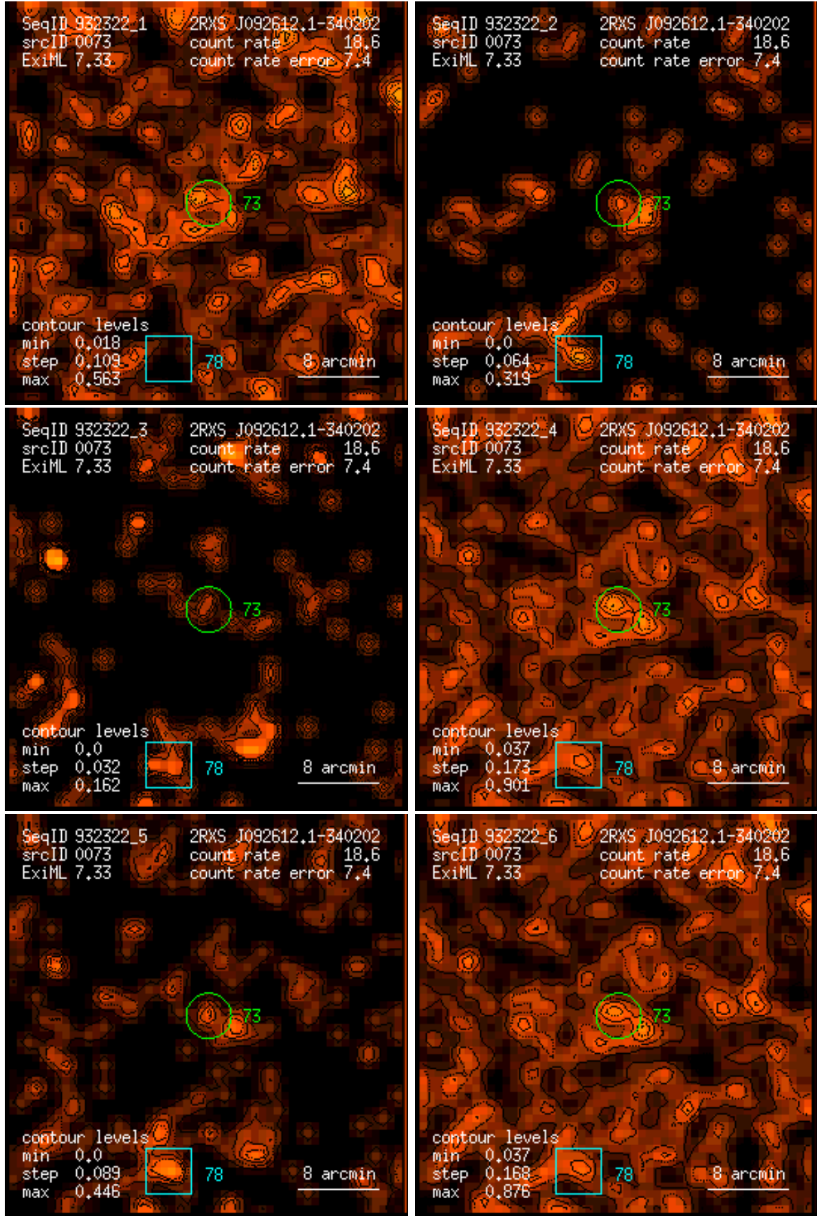
Figure 73: RASS 932322: detection 0073: band rate images, Gaussian filter: (1) PSPC channels 11 – 41, (2) 52 – 90, (3) 91 – 201, (4) 11 – 235, (5) 52 – 201, (6) 11 – 201. Broad band rates in counts/ks. Band rate contour levels in counts/ks/arcmin 2 .
