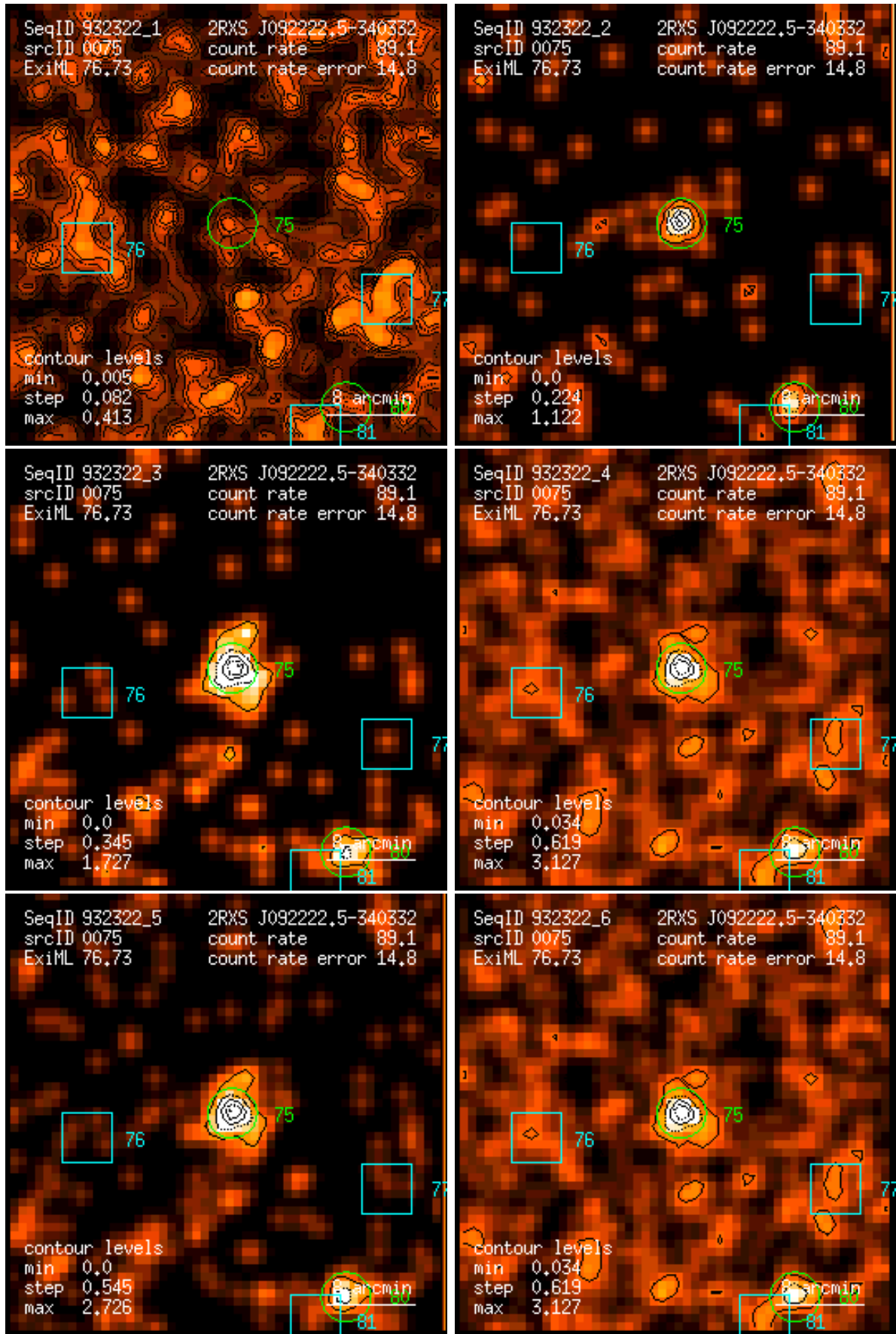
Figure 75: RASS 932322: detection 0075: band rate images, Gaussian filter: (1) PSPC channels 11 – 41, (2) 52 – 90, (3) 91 – 201, (4) 11 – 235, (5) 52 – 201, (6) 11 – 201. Broad band rates in counts/ks. Band rate contour levels in counts/ks/arcmin 2 .
