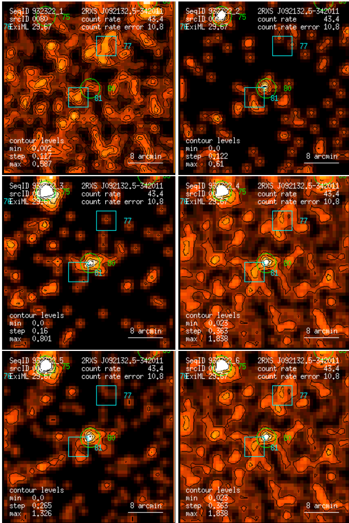
Figure 80: RASS 932322: detection 0080: band rate images, Gaussian filter: (1) PSPC channels 11 – 41, (2) 52 – 90, (3) 91 – 201, (4) 11 – 235, (5) 52 – 201, (6) 11 – 201. Broad band rates in counts/ks. Band rate contour levels in counts/ks/arcmin 2 .
