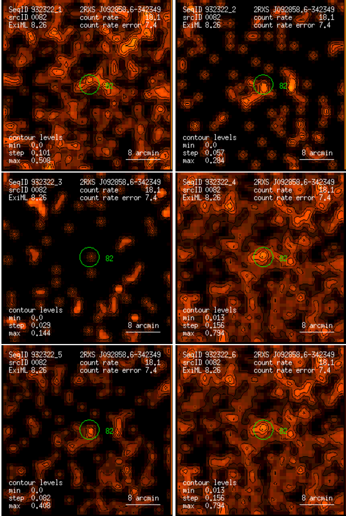
Figure 82: RASS 932322: detection 0082: band rate images, Gaussian filter: (1) PSPC channels 11 – 41, (2) 52 – 90, (3) 91 – 201, (4) 11 – 235, (5) 52 – 201, (6) 11 – 201. Broad band rates in counts/ks. Band rate contour levels in counts/ks/arcmin 2 .
