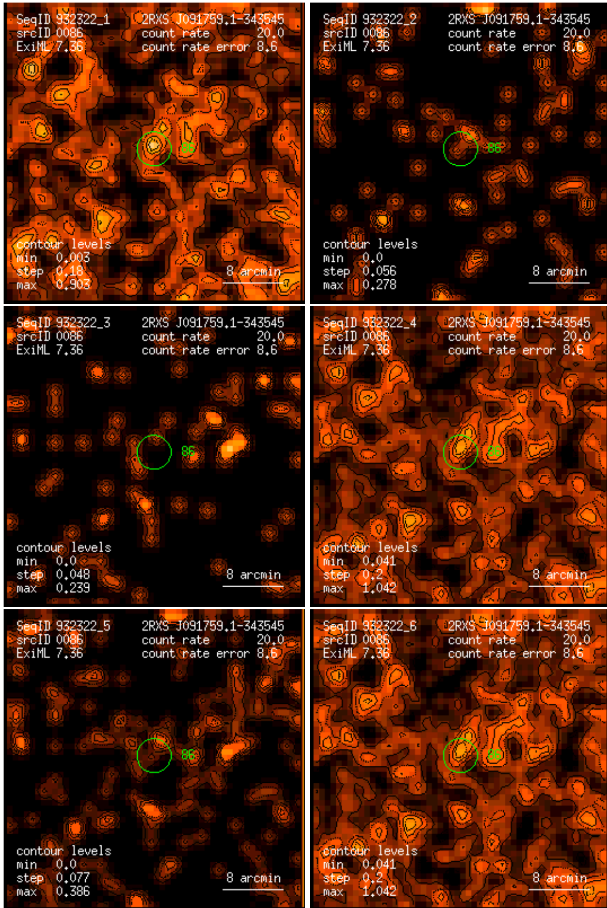
Figure 86: RASS 932322: detection 0086: band rate images, Gaussian filter: (1) PSPC channels 11 – 41, (2) 52 – 90, (3) 91 – 201, (4) 11 – 235, (5) 52 – 201, (6) 11 – 201. Broad band rates in counts/ks. Band rate contour levels in counts/ks/arcmin 2 .
