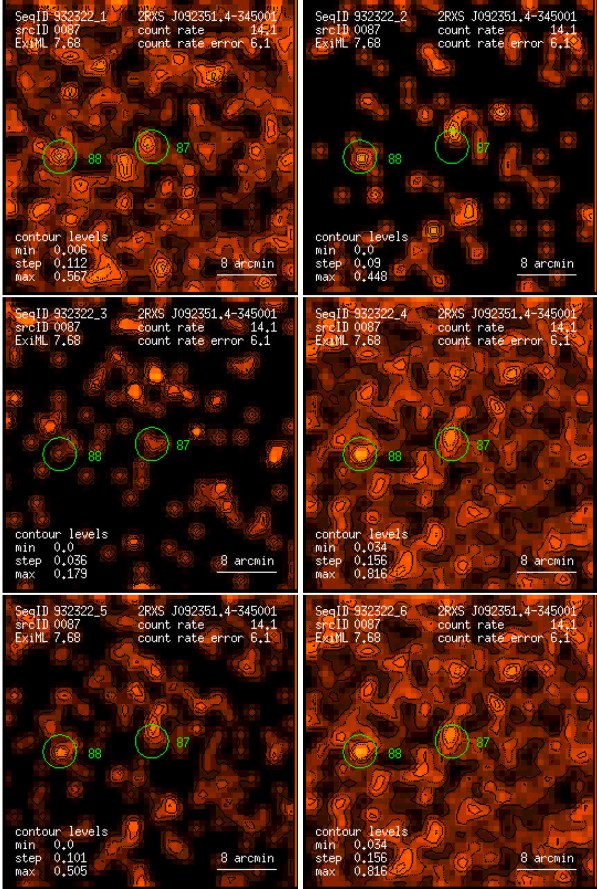
Figure 87: RASS 932322: detection 0087: band rate images, Gaussian filter: (1) PSPC channels 11 – 41, (2) 52 – 90, (3) 91 – 201, (4) 11 – 235, (5) 52 – 201, (6) 11 – 201. Broad band rates in counts/ks. Band rate contour levels in counts/ks/arcmin 2 .
