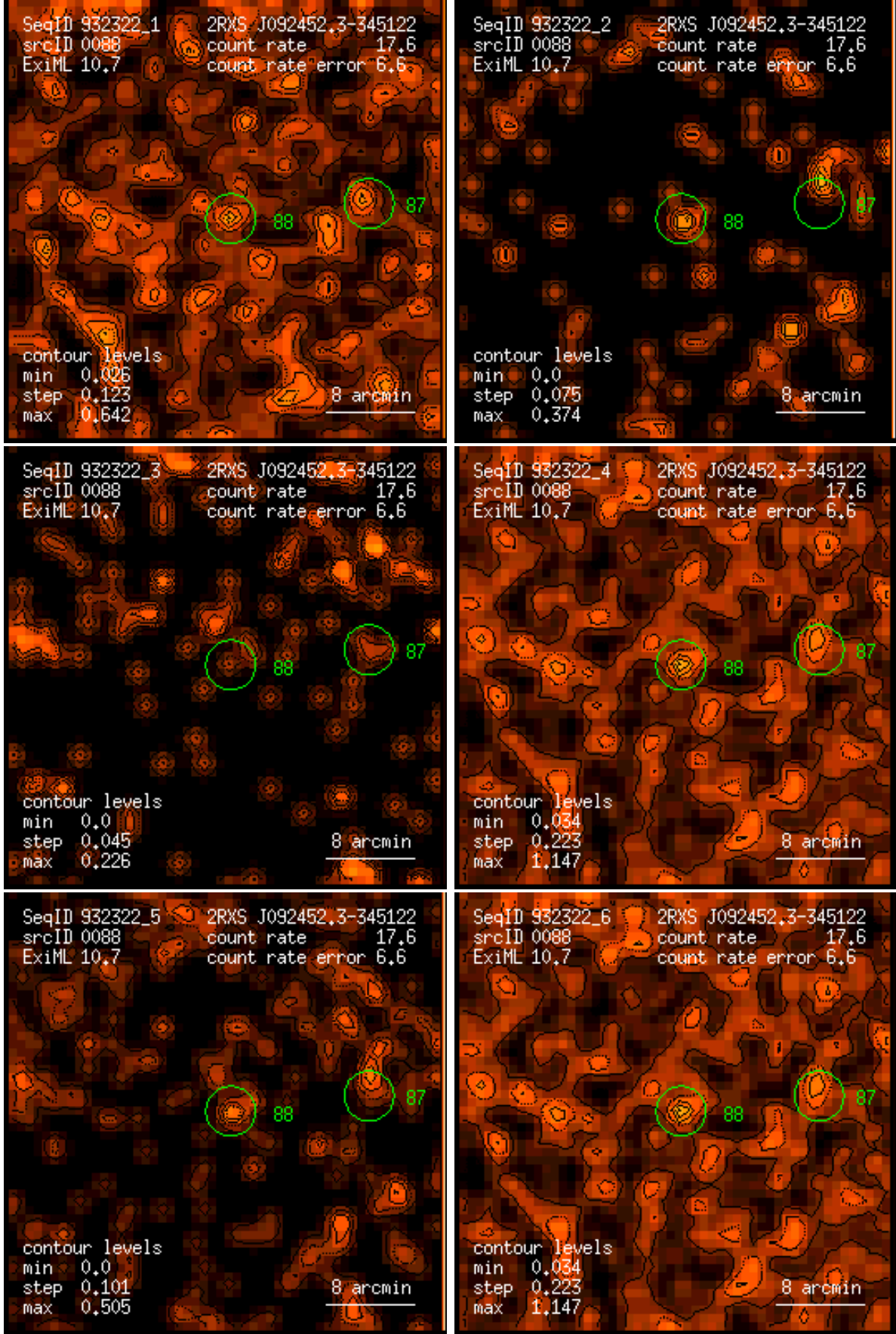
Figure 88: RASS 932322: detection 0088: band rate images, Gaussian filter: (1) PSPC channels 11 – 41, (2) 52 – 90, (3) 91 – 201, (4) 11 – 235, (5) 52 – 201, (6) 11 – 201. Broad band rates in counts/ks. Band rate contour levels in counts/ks/arcmin 2 .
