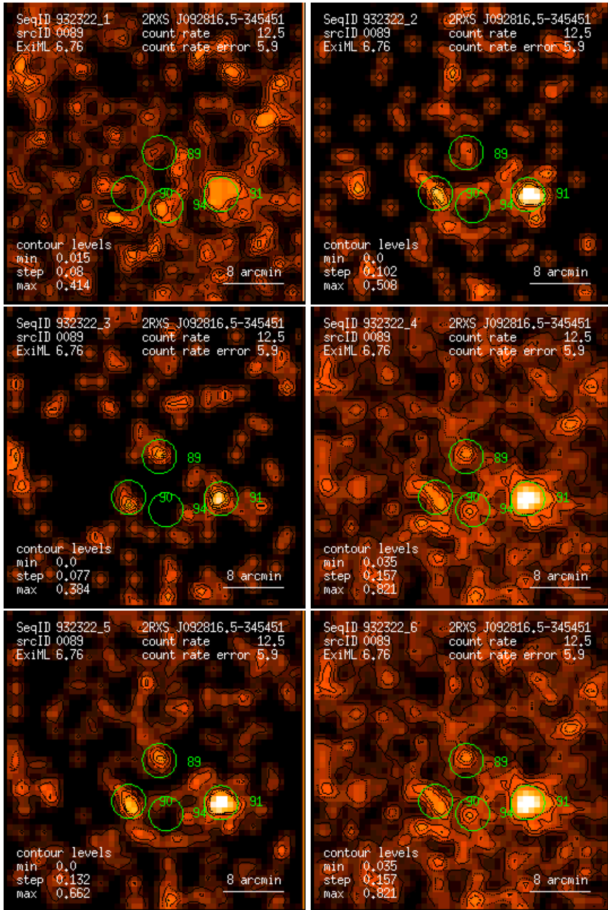
Figure 89: RASS 932322: detection 0089: band rate images, Gaussian filter: (1) PSPC channels 11 – 41, (2) 52 – 90, (3) 91 – 201, (4) 11 – 235, (5) 52 – 201, (6) 11 – 201. Broad band rates in counts/ks. Band rate contour levels in counts/ks/arcmin 2 .
