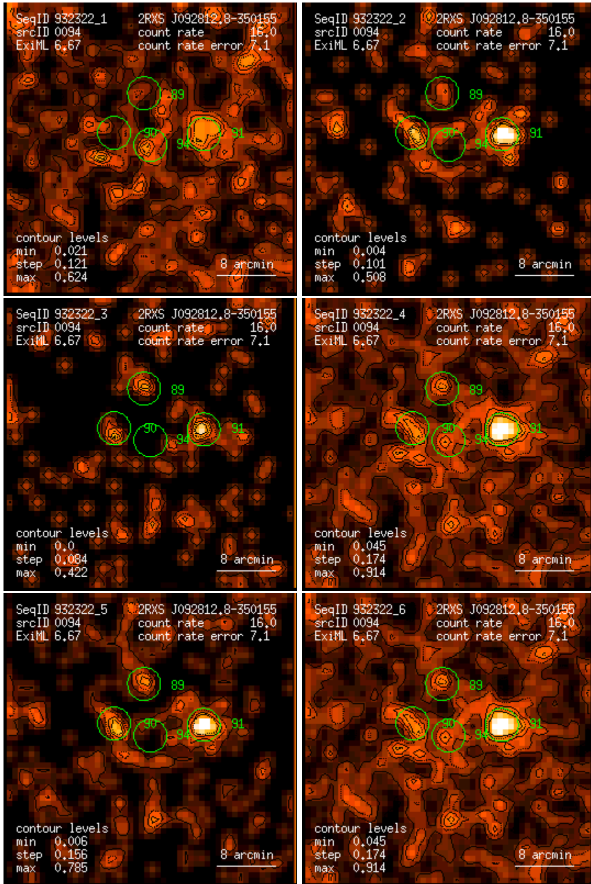
Figure 94: RASS 932322: detection 0094: band rate images, Gaussian filter: (1) PSPC channels 11 – 41, (2) 52 – 90, (3) 91 – 201, (4) 11 – 235, (5) 52 – 201, (6) 11 – 201. Broad band rates in counts/ks. Band rate contour levels in counts/ks/arcmin 2 .
