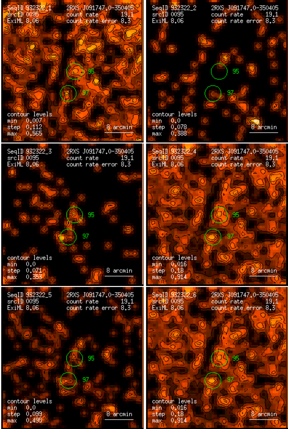
Figure 95: RASS 932322: detection 0095: band rate images, Gaussian filter: (1) PSPC channels 11 – 41, (2) 52 – 90, (3) 91 – 201, (4) 11 – 235, (5) 52 – 201, (6) 11 – 201. Broad band rates in counts/ks. Band rate contour levels in counts/ks/arcmin 2 .
