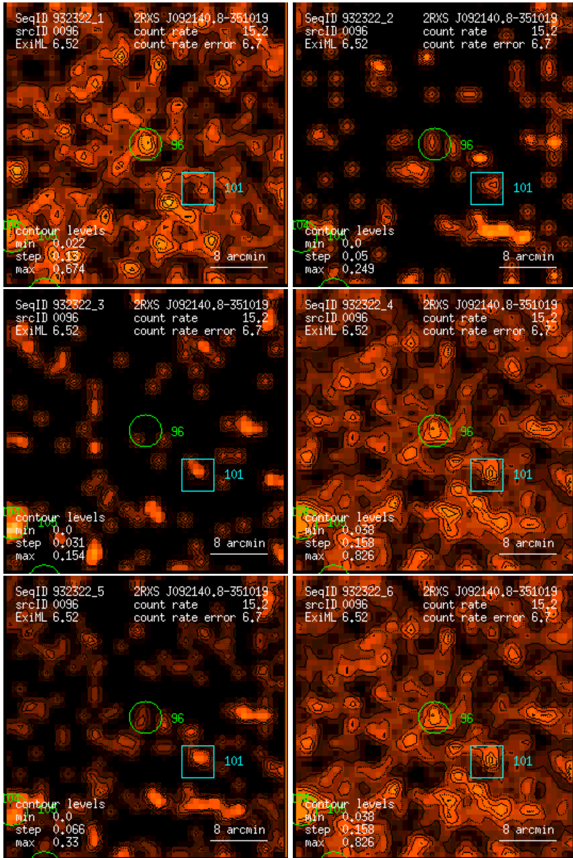
Figure 96: RASS 932322: detection 0096: band rate images, Gaussian filter: (1) PSPC channels 11 – 41, (2) 52 – 90, (3) 91 – 201, (4) 11 – 235, (5) 52 – 201, (6) 11 – 201. Broad band rates in counts/ks. Band rate contour levels in counts/ks/arcmin 2 .
