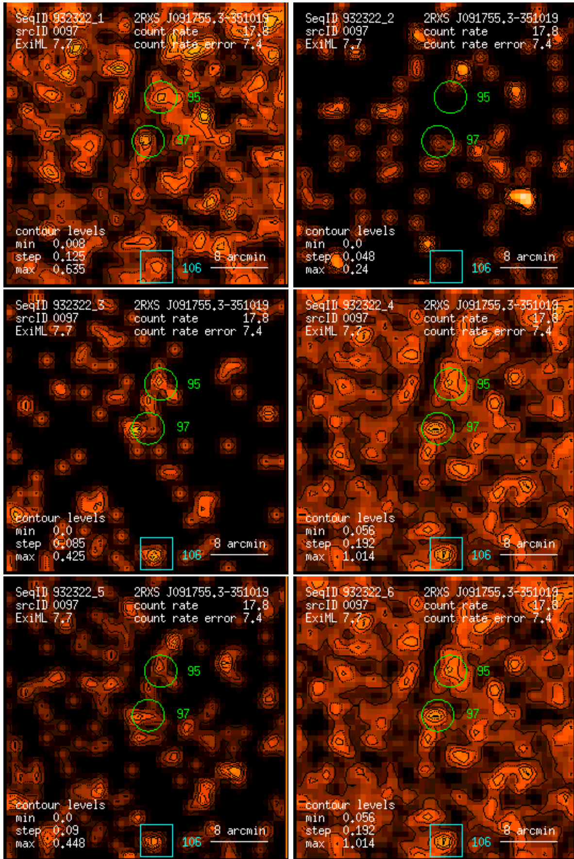
Figure 97: RASS 932322: detection 0097: band rate images, Gaussian filter: (1) PSPC channels 11 – 41, (2) 52 – 90, (3) 91 – 201, (4) 11 – 235, (5) 52 – 201, (6) 11 – 201. Broad band rates in counts/ks. Band rate contour levels in counts/ks/arcmin 2 .
