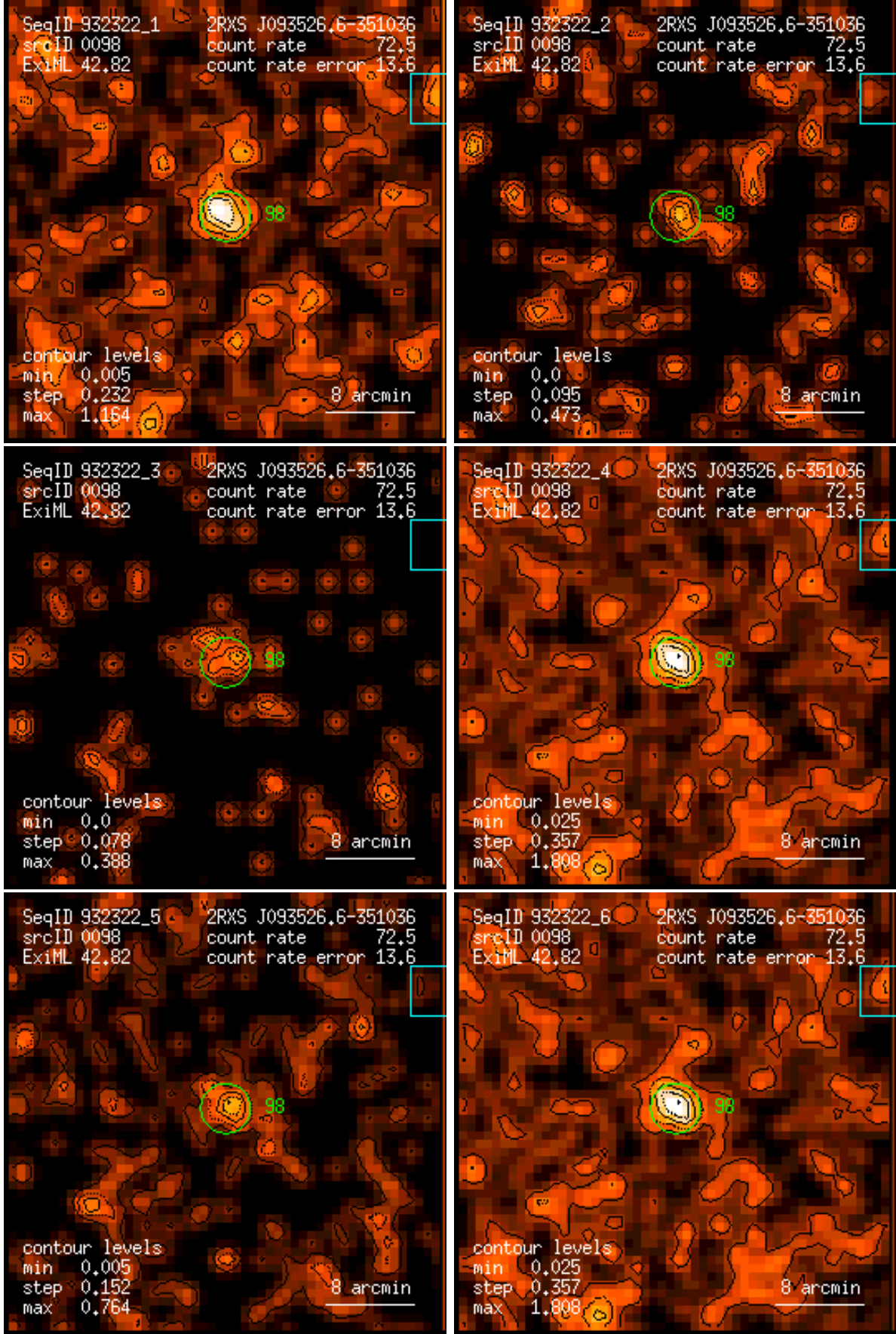
Figure 98: RASS 932322: detection 0098: band rate images, Gaussian filter: (1) PSPC channels 11 – 41, (2) 52 – 90, (3) 91 – 201, (4) 11 – 235, (5) 52 – 201, (6) 11 – 201. Broad band rates in counts/ks. Band rate contour levels in counts/ks/arcmin 2 .
