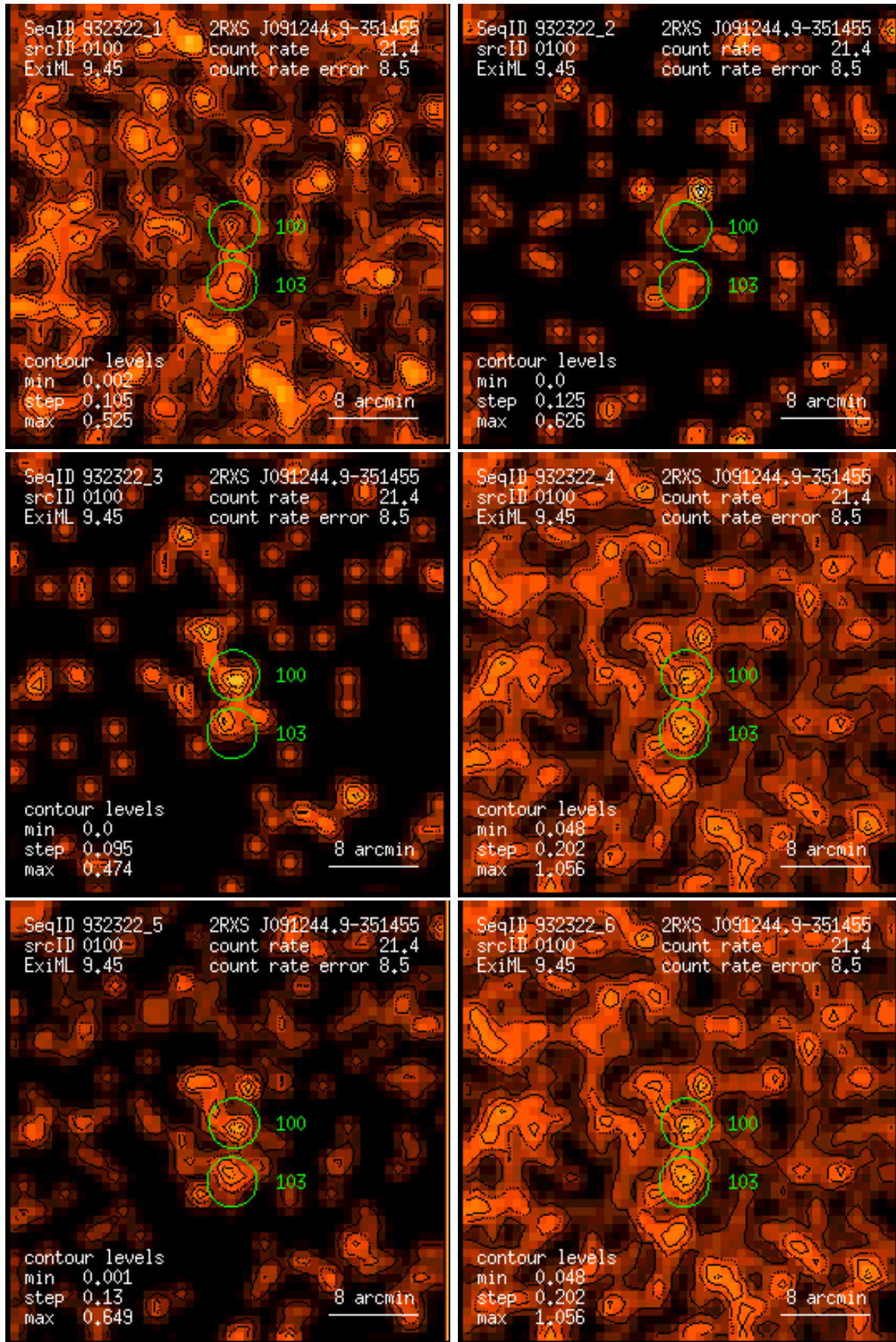
Figure 100: RASS 932322: detection 0100: band rate images, Gaussian filter: (1) PSPC channels 11 – 41, (2) 52 – 90, (3) 91 – 201, (4) 11 – 235, (5) 52 – 201, (6) 11 – 201. Broad band rates in counts/ks. Band rate contour levels in counts/ks/arcmin 2 .
