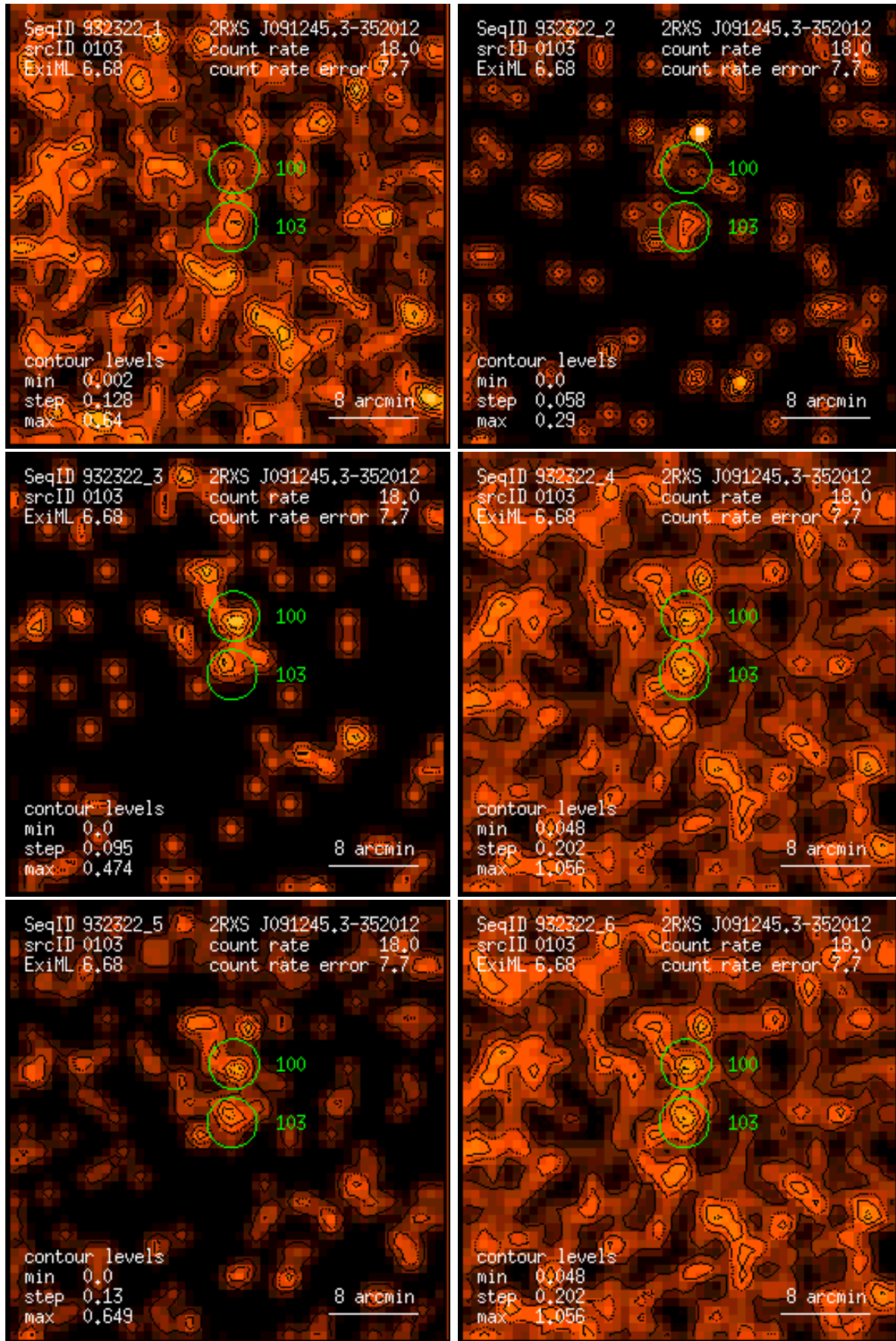
Figure 103: RASS 932322: detection 0103: band rate images, Gaussian filter: (1) PSPC channels 11 – 41, (2) 52 – 90, (3) 91 – 201, (4) 11 – 235, (5) 52 – 201, (6) 11 – 201. Broad band rates in counts/ks. Band rate contour levels in counts/ks/arcmin 2 .
