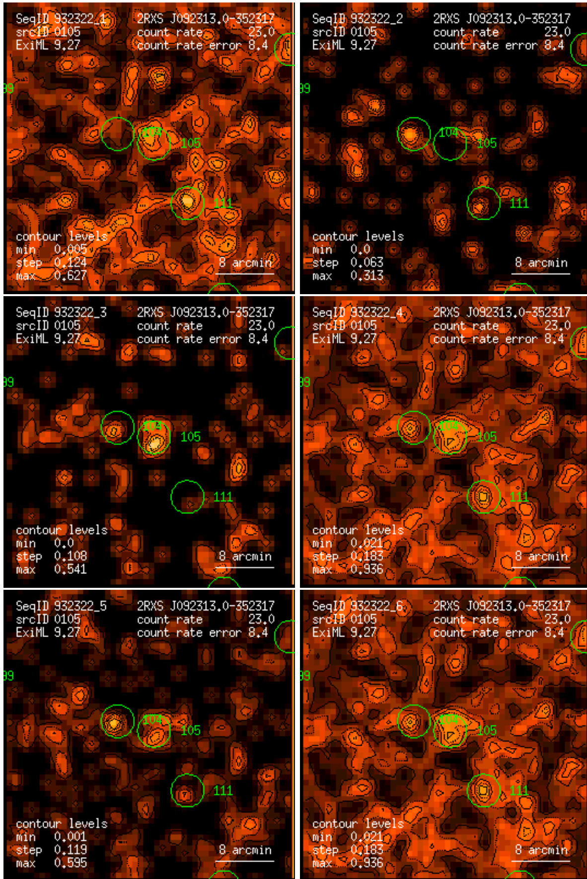
Figure 105: RASS 932322: detection 0105: band rate images, Gaussian filter: (1) PSPC channels 11 – 41, (2) 52 – 90, (3) 91 – 201, (4) 11 – 235, (5) 52 – 201, (6) 11 – 201. Broad band rates in counts/ks. Band rate contour levels in counts/ks/arcmin 2 .
