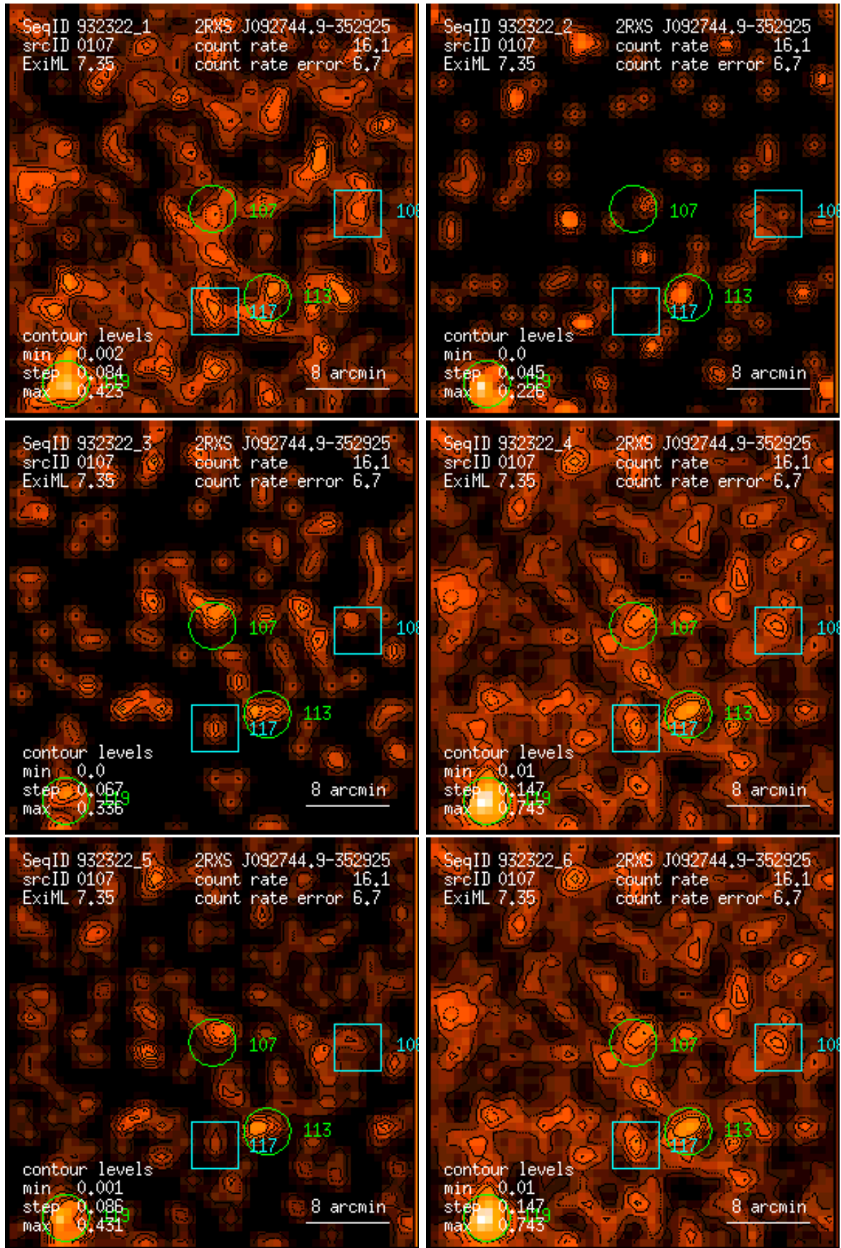
Figure 107: RASS 932322: detection 0107: band rate images, Gaussian filter: (1) PSPC channels 11 – 41, (2) 52 – 90, (3) 91 – 201, (4) 11 – 235, (5) 52 – 201, (6) 11 – 201. Broad band rates in counts/ks. Band rate contour levels in counts/ks/arcmin 2 .
