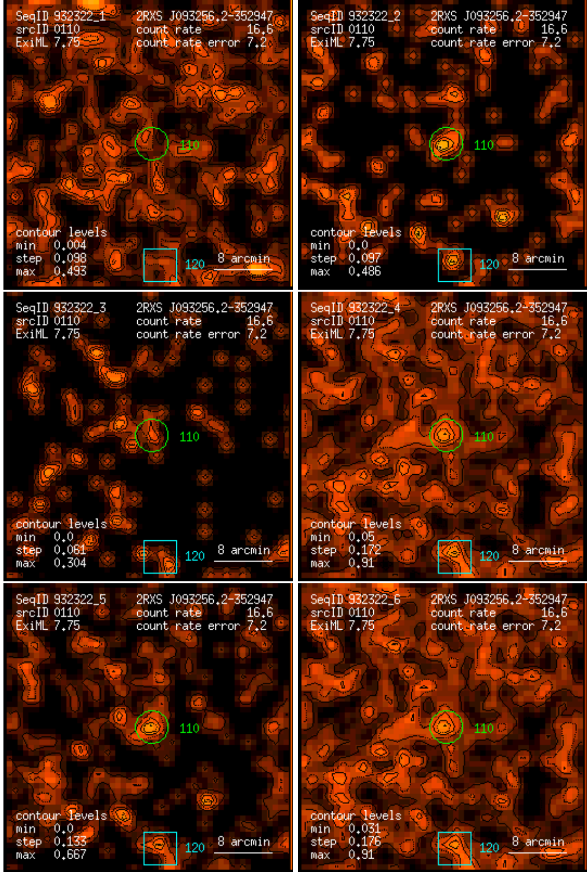
Figure 110: RASS 932322: detection 0110: band rate images, Gaussian filter: (1) PSPC channels 11 – 41, (2) 52 – 90, (3) 91 – 201, (4) 11 – 235, (5) 52 – 201, (6) 11 – 201. Broad band rates in counts/ks. Band rate contour levels in counts/ks/arcmin 2 .
