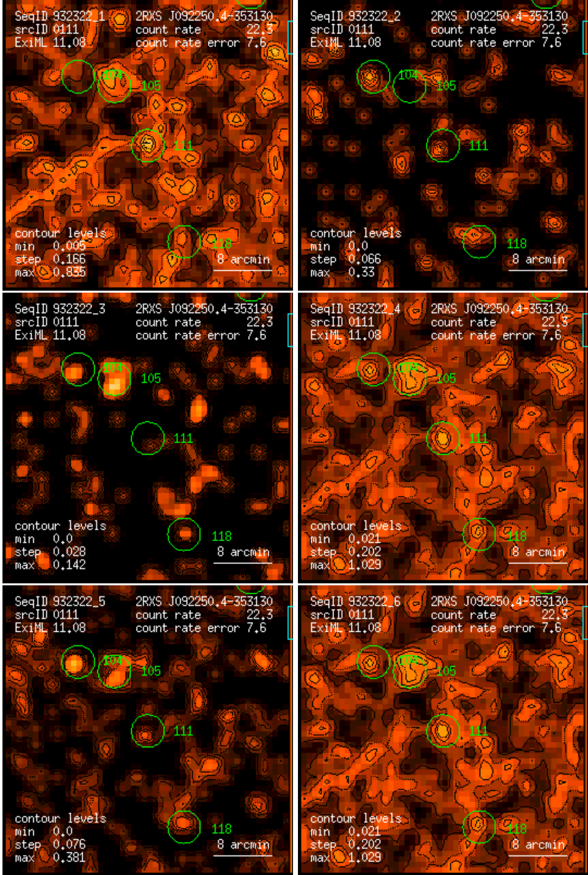
Figure 111: RASS 932322: detection 0111: band rate images, Gaussian filter: (1) PSPC channels 11 – 41, (2) 52 – 90, (3) 91 – 201, (4) 11 – 235, (5) 52 – 201, (6) 11 – 201. Broad band rates in counts/ks. Band rate contour levels in counts/ks/arcmin 2 .
