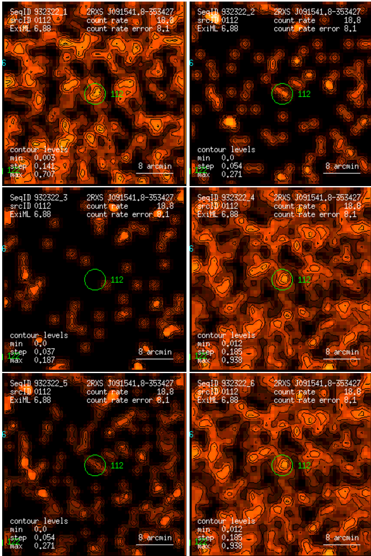
Figure 112: RASS 932322: detection 0112: band rate images, Gaussian filter: (1) PSPC channels 11 – 41, (2) 52 – 90, (3) 91 – 201, (4) 11 – 235, (5) 52 – 201, (6) 11 – 201. Broad band rates in counts/ks. Band rate contour levels in counts/ks/arcmin 2 .
