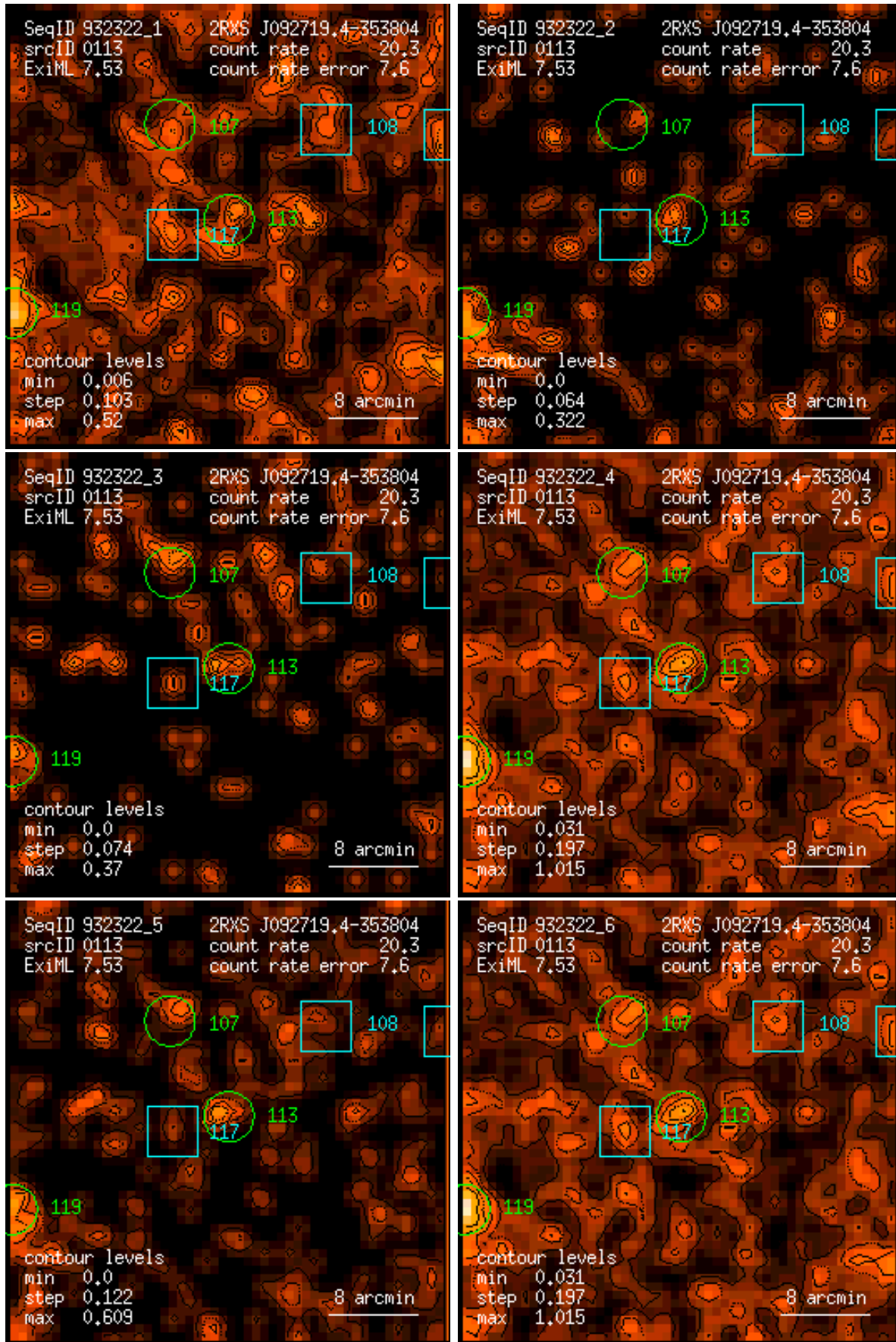
Figure 113: RASS 932322: detection 0113: band rate images, Gaussian filter: (1) PSPC channels 11 – 41, (2) 52 – 90, (3) 91 – 201, (4) 11 – 235, (5) 52 – 201, (6) 11 – 201. Broad band rates in counts/ks. Band rate contour levels in counts/ks/arcmin 2 .
