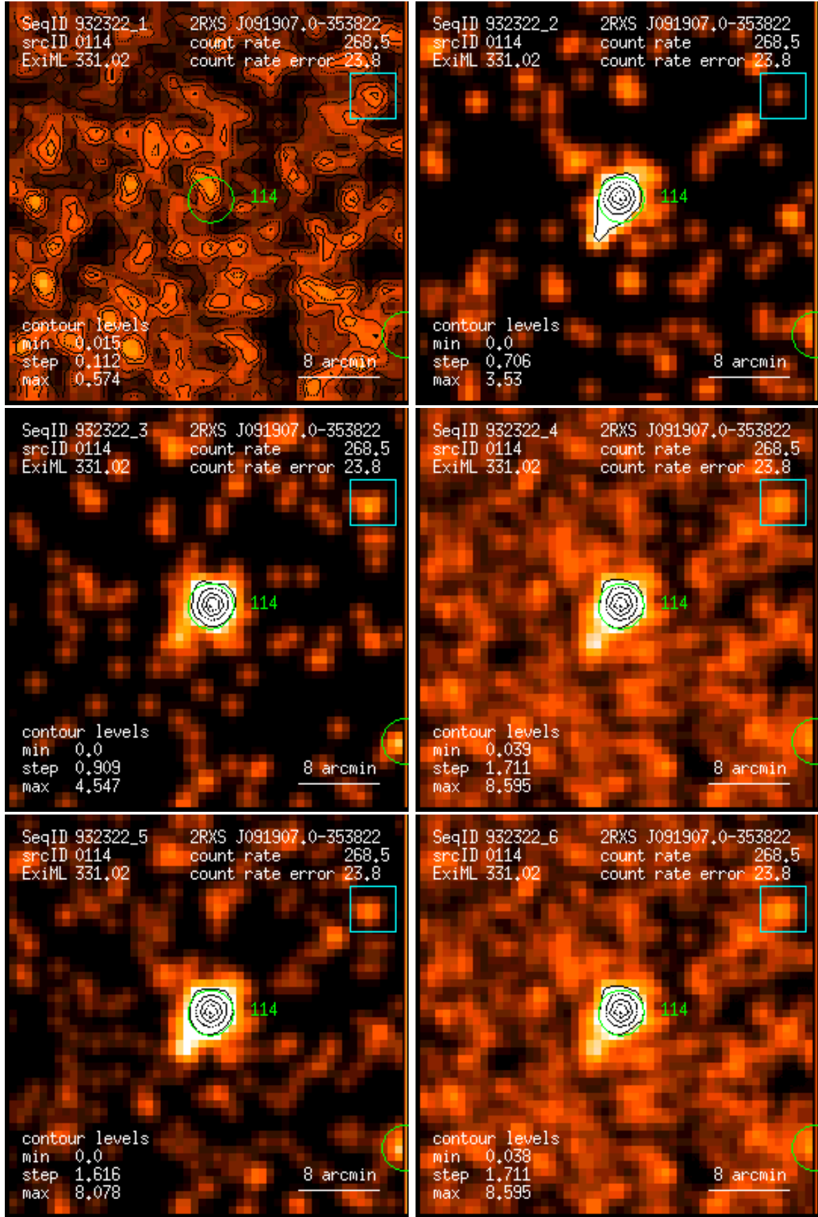
Figure 114: RASS 932322: detection 0114: band rate images, Gaussian filter: (1) PSPC channels 11 – 41, (2) 52 – 90, (3) 91 – 201, (4) 11 – 235, (5) 52 – 201, (6) 11 – 201. Broad band rates in counts/ks. Band rate contour levels in counts/ks/arcmin 2 .
