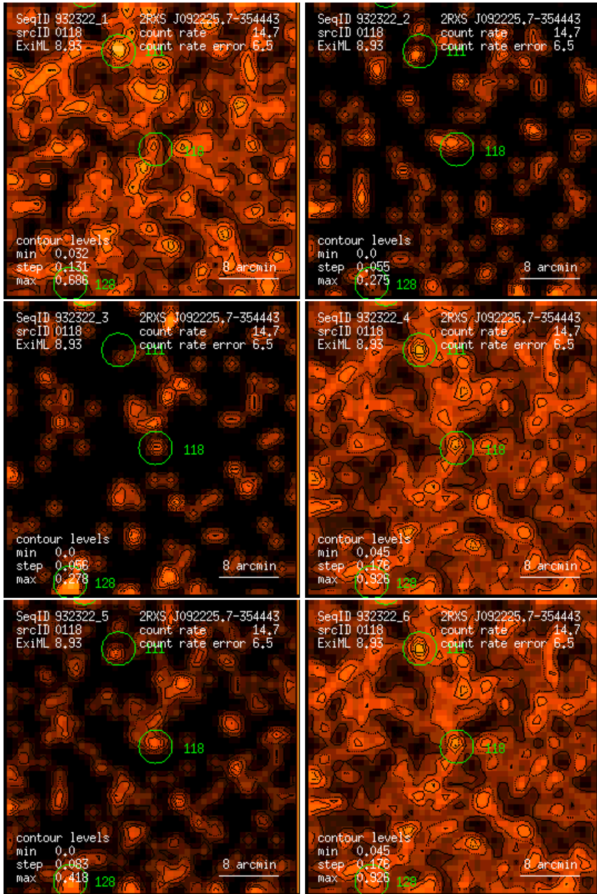
Figure 118: RASS 932322: detection 0118: band rate images, Gaussian filter: (1) PSPC channels 11 – 41, (2) 52 – 90, (3) 91 – 201, (4) 11 – 235, (5) 52 – 201, (6) 11 – 201. Broad band rates in counts/ks. Band rate contour levels in counts/ks/arcmin 2 .
