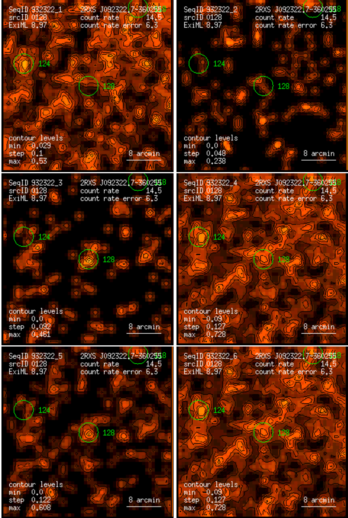
Figure 128: RASS 932322: detection 0128: band rate images, Gaussian filter: (1) PSPC channels 11 – 41, (2) 52 – 90, (3) 91 – 201, (4) 11 – 235, (5) 52 – 201, (6) 11 – 201. Broad band rates in counts/ks. Band rate contour levels in counts/ks/arcmin 2 .
