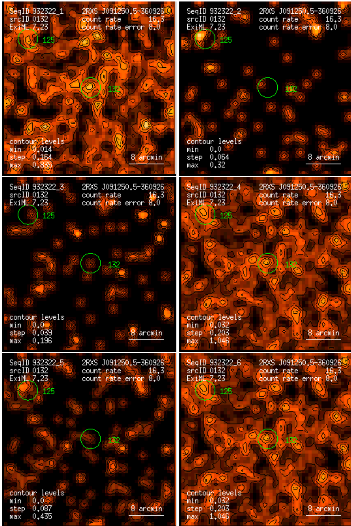
Figure 132: RASS 932322: detection 0132: band rate images, Gaussian filter: (1) PSPC channels 11 – 41, (2) 52 – 90, (3) 91 – 201, (4) 11 – 235, (5) 52 – 201, (6) 11 – 201. Broad band rates in counts/ks. Band rate contour levels in counts/ks/arcmin 2 .
