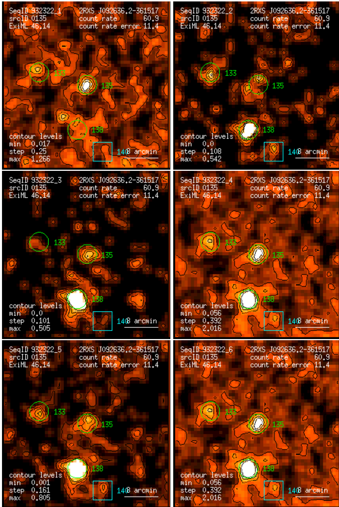
Figure 135: RASS 932322: detection 0135: band rate images, Gaussian filter: (1) PSPC channels 11 – 41, (2) 52 – 90, (3) 91 – 201, (4) 11 – 235, (5) 52 – 201, (6) 11 – 201. Broad band rates in counts/ks. Band rate contour levels in counts/ks/arcmin 2 .
