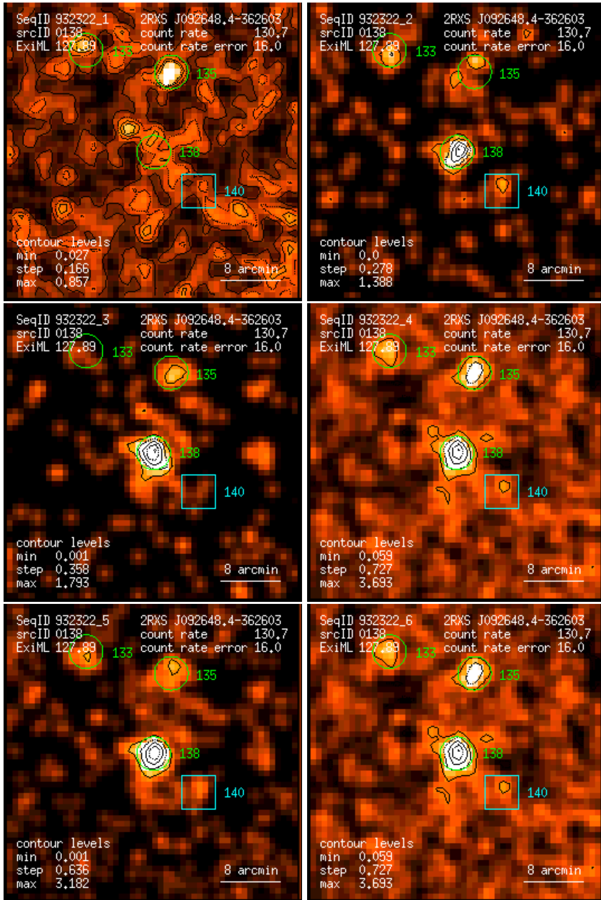
Figure 138: RASS 932322: detection 0138: band rate images, Gaussian filter: (1) PSPC channels 11 – 41, (2) 52 – 90, (3) 91 – 201, (4) 11 – 235, (5) 52 – 201, (6) 11 – 201. Broad band rates in counts/ks. Band rate contour levels in counts/ks/arcmin 2 .
