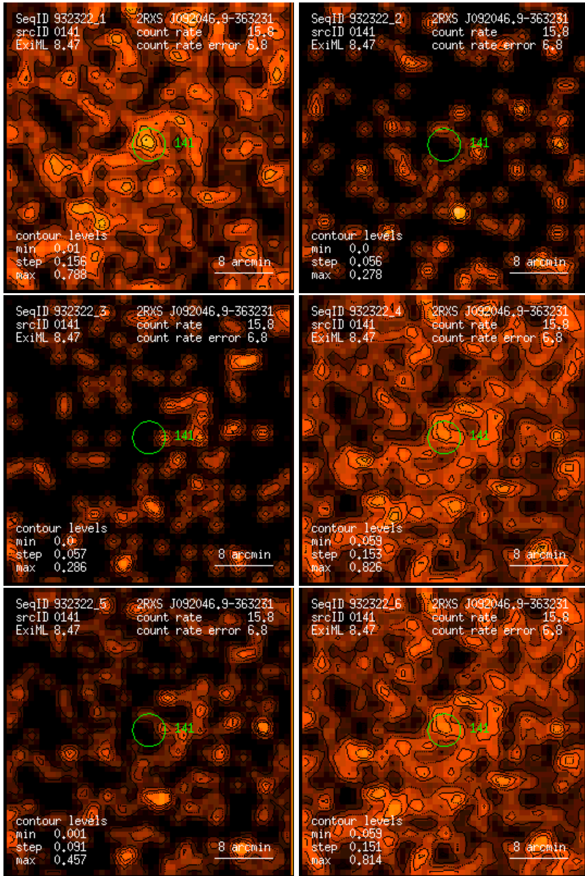
Figure 141: RASS 932322: detection 0141: band rate images, Gaussian filter: (1) PSPC channels 11 – 41, (2) 52 – 90, (3) 91 – 201, (4) 11 – 235, (5) 52 – 201, (6) 11 – 201. Broad band rates in counts/ks. Band rate contour levels in counts/ks/arcmin 2 .
