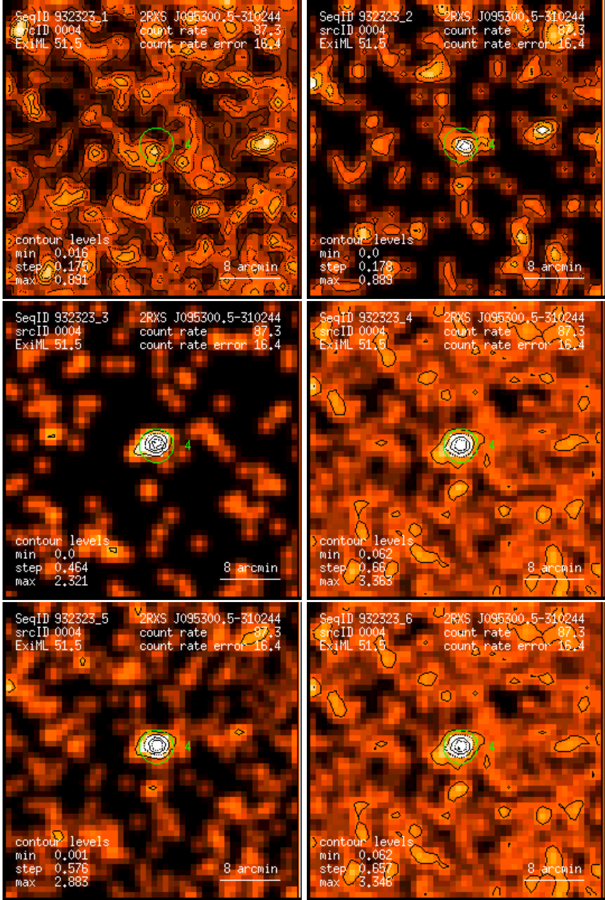
Figure 4: RASS 932323: detection 0004: band rate images, Gaussian filter: (1) PSPC channels 11 – 41, (2) 52 – 90, (3) 91 – 201, (4) 11 – 235, (5) 52 – 201, (6) 11 – 201. Broad band rates in counts/ks. Band rate contour levels in counts/ks/arcmin 2 .
